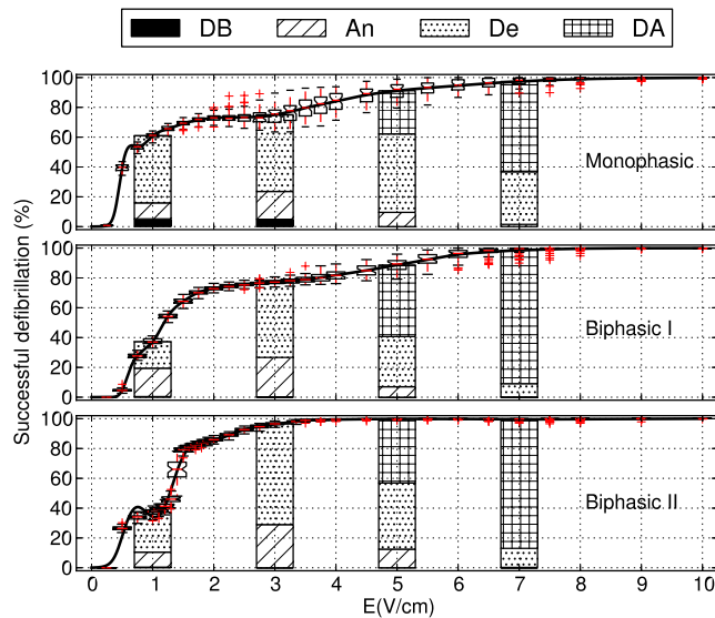
FIG. 4: Four-electrode system. Numerical data (boxplot) and fitted dose-response curve (according to Eq.(7)) for monophasic (top), biphasic I (middle) and biphasic II (bottom) protocol. Stacked bars represent the classification of defibrillation mechanisms for electric fields corresponding to: E=1\text{V/cm} , 3\text{V/cm} , 5\text{V/cm} and 7\text{V/cm} . Here, the abbreviations stand for : DB-direct block, An-annihilation, De-delayed block and DA-direct activation.
