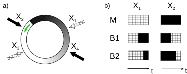
FIG. 2: Illustration of the four-electrode system setup.
