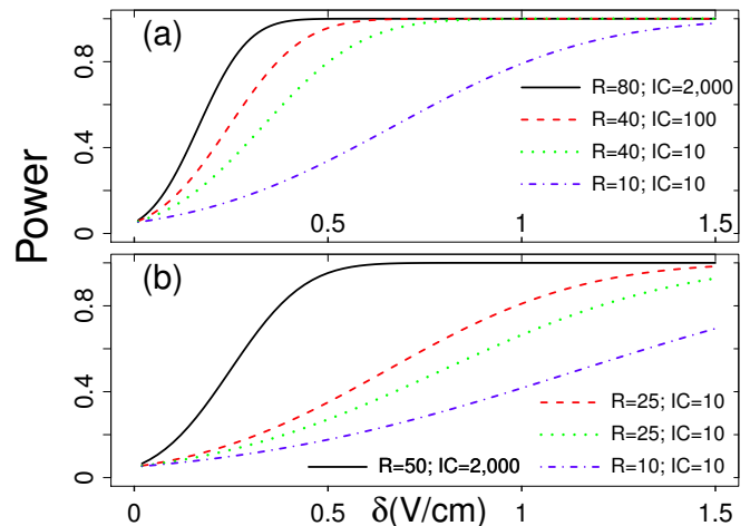
FIG. 9: (Color online) Statistical power calculation for the comparison between the M and B2 protocols (one-tail, \alpha = 0.05 ). (a) two-electrode system (based on the GLM fitting). (b) four-electrode system (based on the GAM fitting). The parameters R and IC indicate the number of rings and initial conditions, respectively.
