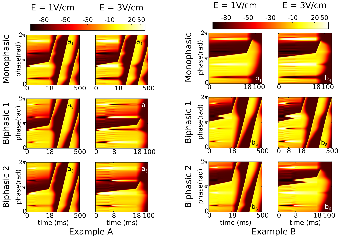
FIG. 7: Space-time plots of V_m for two different initial condition. Example A : \phi_f(t=0) = 2.22\text{rad} and Example B: \phi_f(t=0)=3.27\text{rad} . An external shock is applied during the first 8ms. To highlight the effect of the shock, the time resolution is one order of magnitude larger for t < 18\text{ms} . Space-plots are shown for two shock strengths : E=1\text{V/cm} and E=3\text{V/cm} (columns) and all three protocols (rows). Note that we have used a nonlinear color scale for V_m to enhance clarity.
