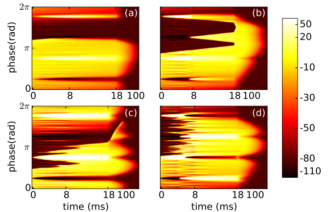
FIG. 5: Space-time plots of V_m showing examples of defibrillation mechanisms. The shock is applied through a four-electrode system. (a) Direct block (Monophasic, E=1 V/cm) (b) Annihilation (Biphasic 2, E=3 V/cm) (c) Delayed block (Monophasic, E=5 V/cm) (d) Direct activation (Biphasic 1, E=7 V/cm). The shock is applied during the first 8ms. The time scale of all the plots is magnified 10 times for t \in (0,18) with respect to t > 18 ms. A nonlinear color scale for V_m is used for all the plots.
