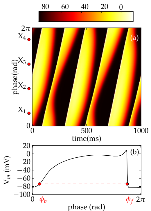
FIG. 1: (Color online) a) Space-time plot of the discordant-alternans wave on the one-dimensional ring. The vertical axis is space ( L = 6.7 cm) and it is rescaled to the phase variable varying in [0, 2\pi] radians. The color-coding quantifies the values of the transmembrane potential V_m in mV units (Top color bar). The locations of the four electrodes X_i ( i=1, \dots, 4 ) are also depicted. b) Snapshot of V_m taken from (a) at time t = 400 ms.
