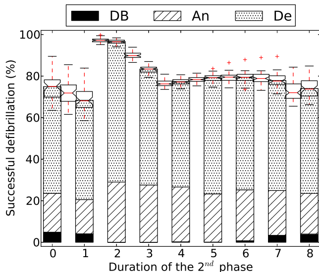
FIG. 8: Dependence of the defibrillation success rate on the duration of the second phase (in ms) for the biphasic protocols. The shock strength is fixed to E=3\text{V/cm} . The total shock duration is also kept fixed at 8 ms.
