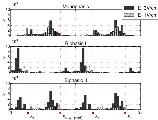
FIG. 6: Histograms showing the number of successful defibrillation trials via the delayed block mechanism. Here \phi_f denotes the position where the blocked front was last detected before being blocked. Histograms are compared for monophasic (upper plot), biphasic 1 (middle plot) and biphasic 2 (lower plot) protocols. Note that the results for E=1\text{V/cm} are depicted with narrower hatched bars for the sake of clarity.
