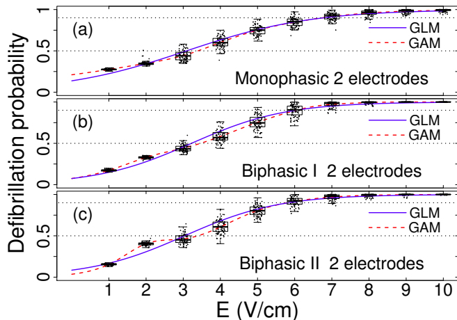
FIG. 3: (Color online) Two-electrode system. Numerical data (boxplot) and fitted dose-response curve (according to Eq.(6) solid blue lines; and Eq.(7) dashed red lines) for monophasic (a), biphasic I (b) and biphasic II (c) protocols.
