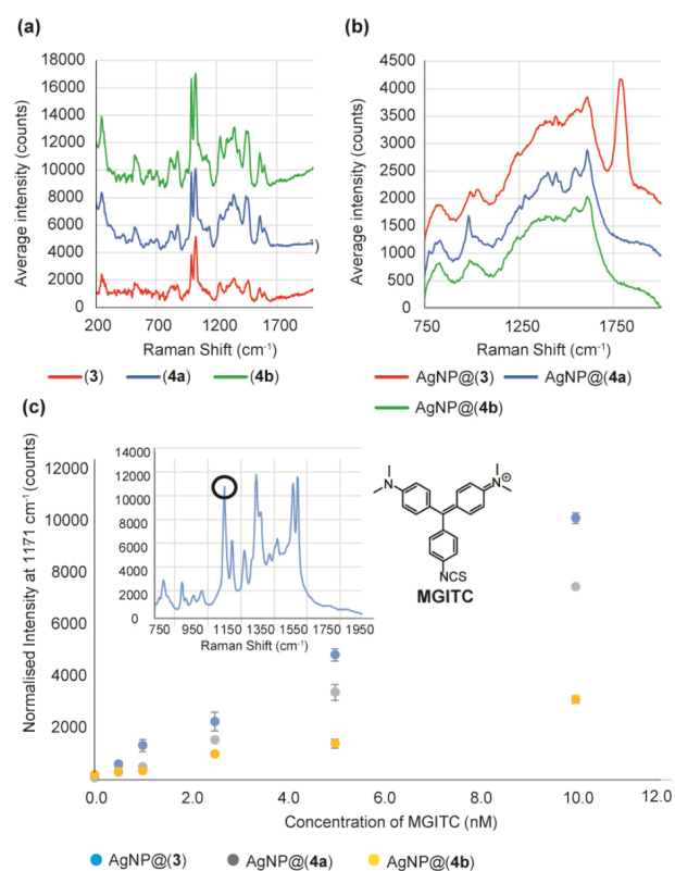
Fig. 3. (a) Stacked Raman spectra of sugar ligands (785 nm excitation; 1 accumulation; 1 s scan ( 3 ); 10 s scan ( 4a ); 5 s scan ( 4b )). (b) Stacked SERS spectra of \text{AgNP}@(\mathbf{3}) , \text{AgNP}@(\mathbf{4a}) and \text{AgNP}@(\mathbf{4b}) (532 nm excitation; 1 s scan; 1 accumulation). (c) Plot of the intensity of the 1171 \text{ cm}^{-1} peak of MGITC using \text{AgNP}@(\mathbf{3}, \mathbf{4a-b}) at decreasing concentrations of MGITC. Inset- SERS spectrum of MGITC using \text{AgNP}@(\mathbf{4a}) highlighting the peak of interest.
