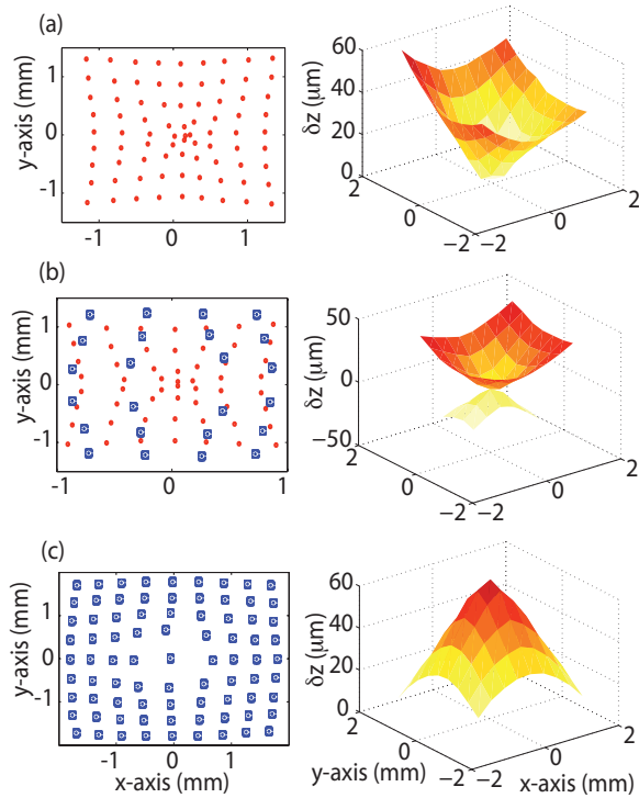
Fig. 3. Left hand side figures: H-S acquisition. Right hand side: corresponding retrieved phase. (a) Beginning of the Bessel zone: z_0 = 18 mm. (b) Middle of the Bessel zone: z_0 = 58 mm. (c) End of the Bessel zone: z_0 = 108 mm. In all figures, the converging front is shown in red circles and the diverging pulse front in blue spots.
