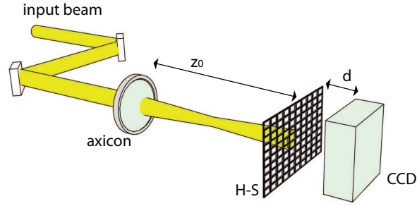
Fig. 1. Experimental layout of the experiment: z_0 indicates the distance between the axicon and the H-S sensor, d indicates the distance between the H-S sensor and the detector. The temporal characterization is performed by substituting the H-S sensor with a FROG setup.
