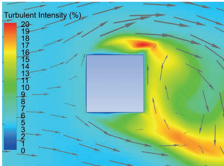
Figure 3: CFD simulation of airflow around cube
