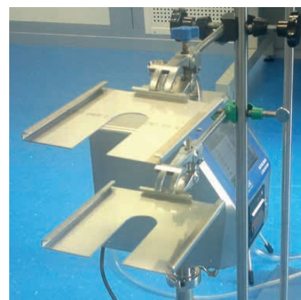
Figure 4: Two parallel witness plate holders with an airborne particle counter in the background
