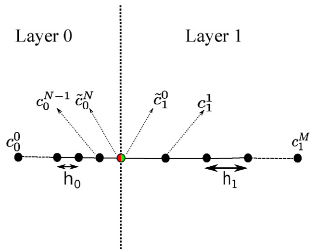
Fig. 4. Illustration of grid nodes in the two layers and the interface points (in red and green). They are computed a posteriori as a linear combination of the neighbouring grid points (Eqs. (6.6)–(6.7)).
