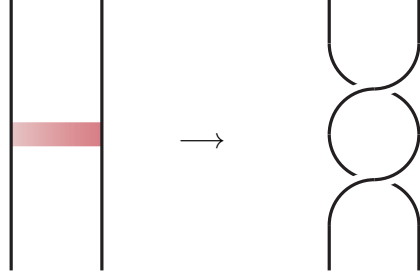
FIGURE 1. Encoding a crossing change with a band.
