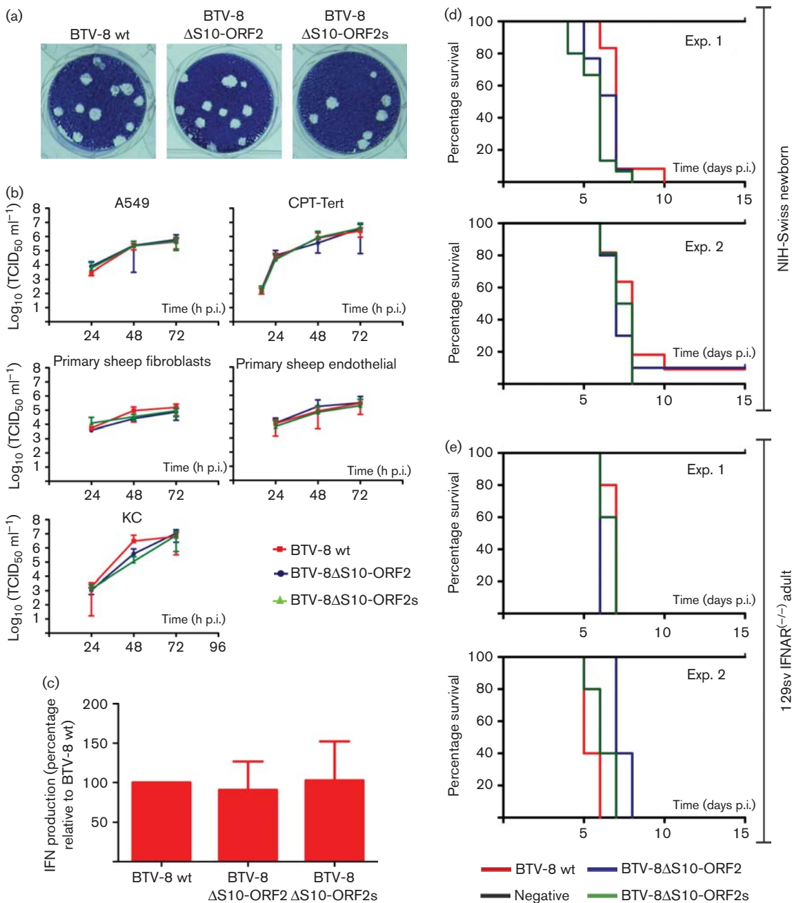
Fig. 6. Replication kinetics and virulence of BTV8ΔS10-ORF2 viruses. (a) Plaques induced by BTV8ΔS10-ORF2, BTV8ΔS10-ORF2s and wt BTV-8 in CPT-Tert cells. (b) Replication kinetics of BTV8ΔS10-ORF2 (blue), BTV8ΔS10-ORF2s (green) and wt BTV-8 (red) in various cell types as indicated. Cells were infected with a m.o.i. of 0.001 or 0.01 as described in Methods. Supernatants were harvested at 24, 48 and 72 h post-infection and titres determined by limiting dilution in BSR cells and expressed as \log_{10}(\text{TCID}_{50} \text{ ml}^{-1}) . Each experiment was performed independently, three times, using two independently generated virus stocks. (c) Interferon response of oVEC to BTV-8 wt, BTV8ΔS10-ORF2 and BTV8ΔS10-ORF2s infection. (d) Three- to four-day-old NIH-Swiss newborn mice ( n=10-15 ) were infected intracerebrally with 300 p.f.u. of the indicated viruses. Top panel, experiment 1 (log rank test, P=0.0001 ). Bottom panel, experiment 2 (log rank test, P=0.0024 ). (e) Adult IFNAR -/- ( n=5 ) were infected intraperitoneally with 100 p.f.u. of the indicated viruses. Top panel, experiment 1 (log rank test, P=0.0226 ). Bottom panel, experiment 2 (log rank test, P=0.0014 ). (b-c) Error bars represent the SD from three independent experiments.
