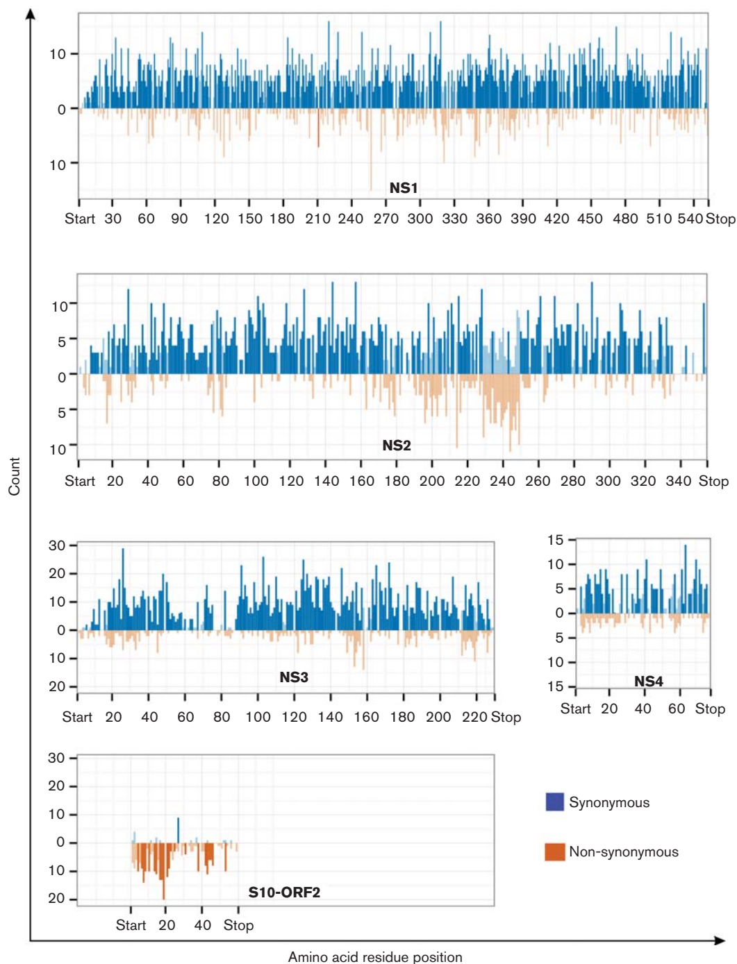
Fig. 2. Frequency of synonymous vs non-synonymous changes in BTv non-structural proteins. Observed synonymous (blue) and non-synonymous (gold) changes determined by the SLAC method for NS1, NS2, NS3, NS4 and S10-ORF2 ORFs. Codons with significantly higher synonymous and non-synonymous changes than expected are shown in dark blue and dark gold bars, respectively. Bars with lighter colours represent values not reaching significance.
