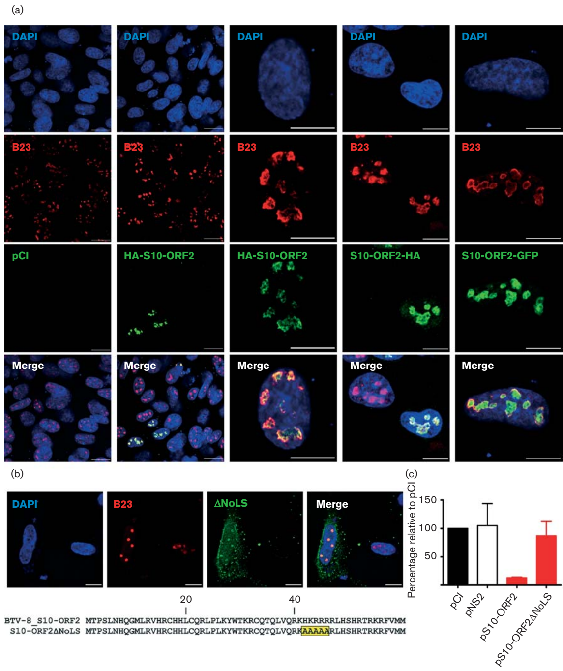
Fig. 4. Localization of S10-ORF2 in transfected cells. (a) CPT-Tert cells were transfected with a series of constructs expressing S10-ORF2 fused at either the N- or C-terminal with HA or GFP (only at the C-terminal) or an empty pCI vector. Cells were fixed 24 h post-transfection and analysed by confocal microscopy using antibodies against the nucleolar protein B23 (in red) and HA (in green). Nuclei were stained with DAPI. Bars correspond to 20 μm for the top two rows and 10 μm for the bottom two rows. (b) Mutations of the predicted nucleolar localization signal (NoLS) within S10-ORF2. CPT-Tert cells were transfected with pS10-ORF2ΔNoLS and analysed by immunofluorescence as described above (bars, 10 μm). (c) Effect of S10-ORF2ΔNoLS in reporter assays as described in Methods. Values (%) relative to the pCI-empty control are plotted. Error bars represent the SD from three independent experiments.
