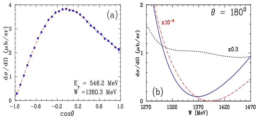
FIG. 10: (Color online) (a) present results for the \gamma p \rightarrow \pi^0 p differential cross section (blue full circles) at E_\gamma = 546 MeV ( W = 1380 MeV) fitted with Legendre polynomials (red dashed line); (b) the new SAID PR15 solution (blue solid line) for \pi^0 production angle \theta = 180^\circ ( \cos\theta = -1 ) as a function of the c.m. energy W , compared with a similar \pi^- p \rightarrow \pi^0 n prediction (rescaled by a factor 10^{-3} ) from SAID WI08 [33] (red dashed line) and a \gamma p \rightarrow \pi^+ n prediction (rescaled by a factor 0.3) from SAID PR15 (black dashed line).
