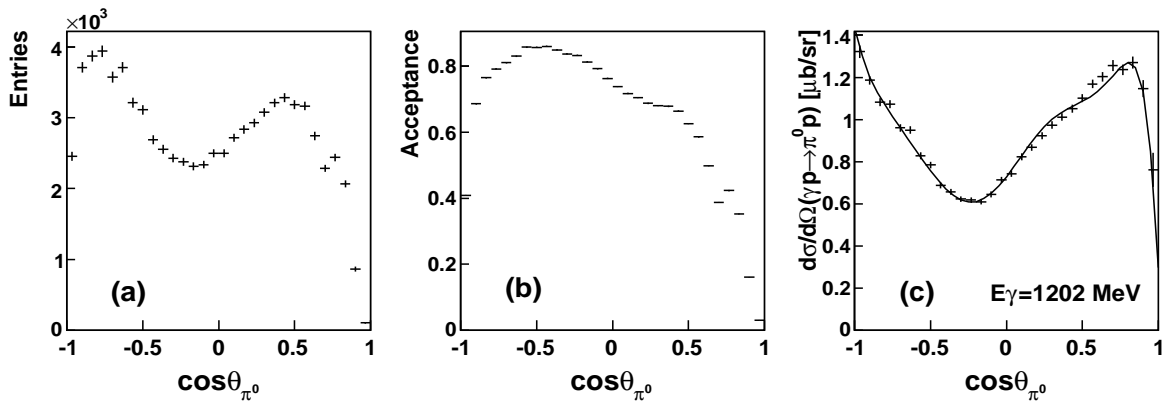
FIG. 2: Same as Fig. 1, but for E_\gamma = 1202 MeV ( W=1771 MeV).
