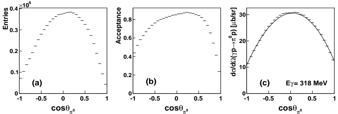
FIG. 1: \cos \theta distributions for \gamma p \rightarrow \pi^0 p , with \theta being the angle between the directions of the outgoing \pi^0 and the incident photon in the c.m. frame, obtained for E_\gamma = 318 MeV ( W=1215 MeV): (a) experimental data after subtraction of the empty-target and the random background; (b) angular acceptance obtained from the MC simulation of \gamma p \rightarrow \pi^0 p ; (c) results for the \gamma p \rightarrow \pi^0 p differential cross section compared to the prediction by SAID [23] with its CM12 [24] solution. The error bars on all data points represent statistical uncertainties only.
