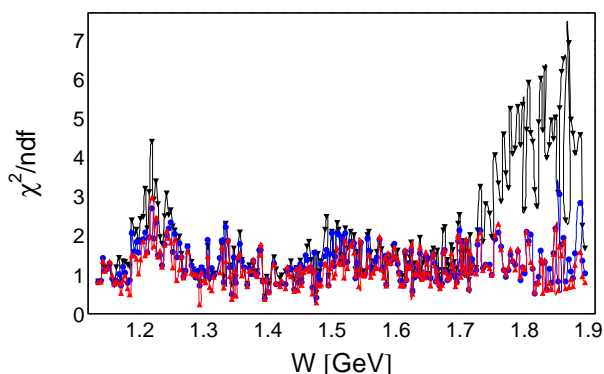
FIG. 11: (Color online) Energy dependence of the reduced \chi^2 values for Legendre fits of the present \gamma p \rightarrow \pi^0 p differential cross sections with j_{\max} = 6 (black triangles down), 8 (blue circles), and 10 (red triangles up), where the angular-dependent systematic uncertainties were not taken into account.
