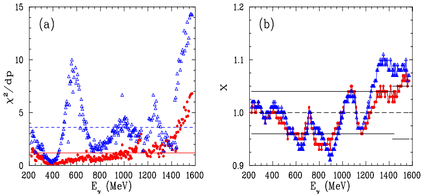
FIG. 8: (Color online) Comparison of the previous SAID solution DU13 [5] (blue open triangles) applied to the present data and the new SAID PR15 solution (red full circles) obtained after adding the present data into the fit for: (a) \chi^2/\text{dp} values averaged only within each energy bin E_\gamma , where the horizontal lines (blue dashed for DU13 and red solid for PR15) show the corresponding \chi^2/\text{dp} values from Table I; (b) results for the normalization parameter X as a function of E_\gamma , where the horizontal solid lines show the deviations (from the dashed line at X = 1 ) equal to the magnitude of the overall systematic uncertainties, which are 4% and 5% for the data from Run-I and Run-II, respectively.
