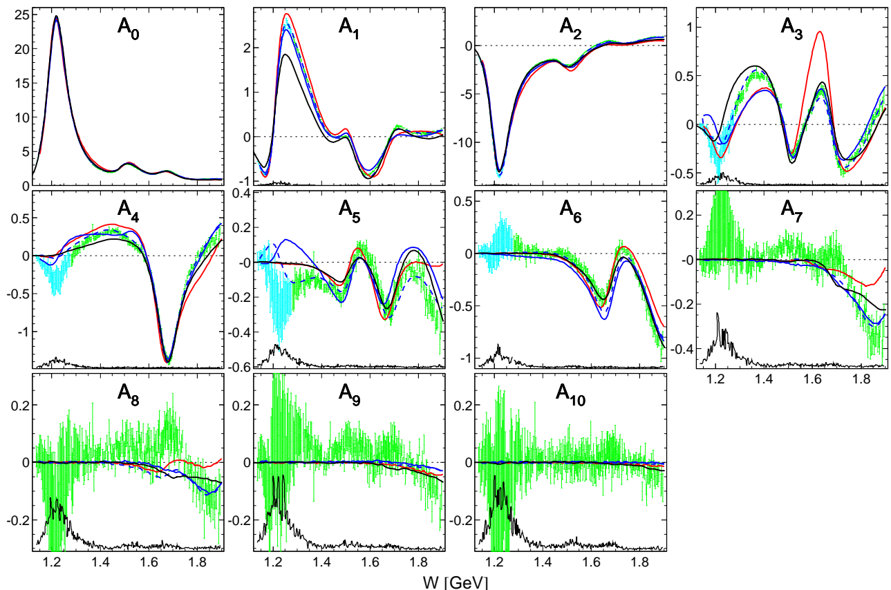
FIG. 12: (Color online) Coefficients A_j (in \mu\text{b}/\text{sr} units) obtained from fitting the present \gamma p \rightarrow \pi^0 p differential cross sections with Legendre polynomials up to order six (cyan points) and ten (green points), compared to the results of the Legendre-polynomial fits ( j_{\text{max}} = 10 ) made to the predictions generated from SAID CM12 [24] (blue solid line), MAID2007 [30] (red solid line), BG2014-02 [31] (black solid line), and SAID PR15 (blue dashed line). The error bars on all points represent A_j uncertainties from the fits with using only the statistical uncertainties. A black histogram at the bottom of each plot shows the systematic uncertainty in A_j caused by the angular-dependent systematics in the differential cross sections.
