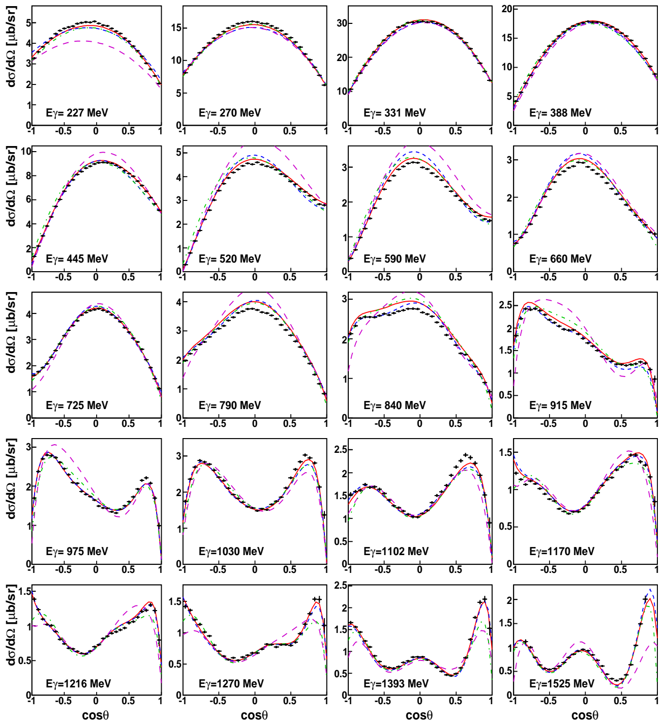
FIG. 7: (Color online) Selected results of this work (black points) for the \gamma p \rightarrow \pi^0 p differential cross sections compared to existing PWA solutions from SAID CM12 [24] (blue dashed line), MAID2007 [30] (magenta long-dashed line), and Bonn-Gatchina BG2014-02 [31] (green dash-dotted line) and to a new SAID PR15 solution (red solid line) obtained after adding the present data points into the fit. The error bars on all data points represent statistical uncertainties only.
