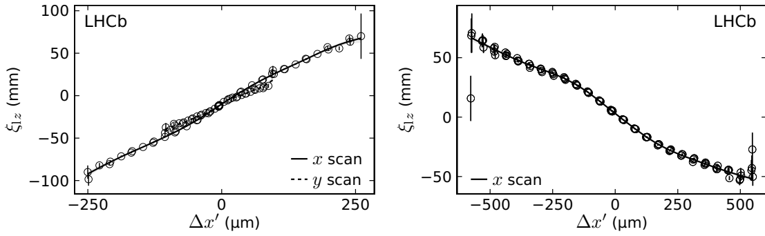
Figure 53. Longitudinal position of the luminous region as function of separation in the crossing plane for reference scans in the (left) April and (right) July VDM sessions. It is assumed that there is no significant orbit and z_{\text{rf}} drift during the reference scans. The data for each scan direction are fitted with a smooth function. In July the crossing plane is orthogonal to the y axis, thus \xi_{lz} is not expected to change during the y scans and the data are omitted. The non-linearity of the curves is due to second order effects, which are not expected for pure Gaussian beams.
