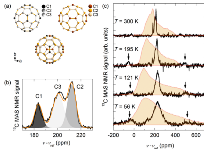
Figure 1: (a) Two equally populated standard \text{C}_{60} orientations (top) related by a 90^\circ rotation about the [001] or equivalently by 44^\circ 23' about the [111] crystal axes in the Fm\bar{3}m average structure of \text{Cs}_3\text{C}_{60} (bottom). Carbon atoms at (0, 0.0491, 0.2407), (0.2051, 0.0767, 0.0987) and (0.1764, 0.1533, 0.0503) crystallographic positions contributing to C1, C2 and C3 ^{13}\text{C} MAS NMR peaks are marked for both standard orientations, respectively. (b) ^{13}\text{C} MAS NMR spectrum measured at room temperature (solid black line) and its fit to three Gaussian components in the intensity ratio, C1:C2:C3 = 1:2:2 (orange line; the grey shaded areas depict the C1, C2, and C3 spectral components). (c) Temperature dependence of the ^{13}\text{C} MAS NMR spectra of fcc \text{Cs}_3\text{C}_{60} . The corresponding static ^{13}\text{C} NMR spectra (shaded areas – data taken from Ref. 4) are shown for comparison. Spinning sidebands (marked with arrows) on both sides of the center band resonance are visible below \sim 200 K.
