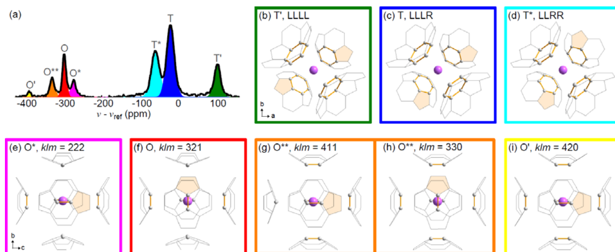
Figure 2: Splitting of ^{133}\text{Cs} MAS NMR spectra ( \nu_{\text{R}} = 25 kHz) of fcc \text{Cs}_3\text{C}_{60} due to the merohedral disorder. The assignment of the high-resolution ^{133}\text{Cs} MAS NMR peaks measured at room temperature (a) to different tetrahedral (b-d) and octahedral site (e-i) coordinations. In (b), the tetrahedral \text{Cs}^+ ion lies directly above the centers of four hexagonal faces of neighboring \text{C}_{60}^{3-} ions which adopt the same standard orientation (configuration LLLL). In (c), one of the \text{C}_{60}^{3-} ions is in the second standard orientation (configuration LLLR). The additional distinct configuration (LLRR, two \text{C}_{60}^{3-} ions in each of the two standard orientations) for the tetrahedral \text{Cs}^+ - \text{C}_{60}^{3-} contacts is depicted in (d). In (e), the octahedral \text{Cs}^+ ion lies directly above the midpoints of six 6:6 bonds of neighboring \text{C}_{60}^{3-} ions which adopt the same standard orientation (configuration 222). In (f), one of the \text{C}_{60}^{3-} ions is in the second standard orientation (configuration 321). The three additional distinct configurations (330, 411, and 420) for the octahedral \text{Cs}^+ - \text{C}_{60}^{3-} contacts are depicted in (g-i).
