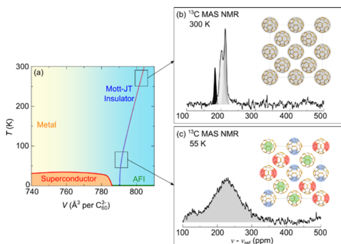
Figure 4: (a) Electronic phase diagram of fcc \text{A}_3\text{C}_{60} fullerides shown as a function of volume occupied per \text{C}_{60}^{3-} ion. The red solid line shows the superconducting transition temperature, T_c and the green solid line the antiferromagnetic ordering temperature, T_N . 4 The dotted line delineates the temperature evolution of the volume occupied per \text{C}_{60}^{3-} ion in fcc \text{Cs}_3\text{C}_{60} at ambient pressure 4 and marks the path along which the present temperature-dependent MAS NMR measurements were undertaken. The line is color-coded to indicate how the correlation time for the Jahn-Teller deformational dynamics compare with the time-scale of the MAS NMR experiments ( 10^{-5} s) – at high-temperatures, this timescale is significantly shorter (red color) but as the temperature is lowered it becomes longer (blue color). Open rectangles mark two representative regions of the phase diagram, where the MAS NMR results reveal different dynamics of the Jahn-Teller effect as depicted in (b) and (c). (b) At high temperatures in the Mott-Jahn-Teller-insulating phase , 53 the rate of interconversion between different Jahn-Teller conformers is very fast on the NMR time-scale (orbital-liquid state) thus restoring the high symmetry of the \text{C}_{60}^{3-} site and allowing for the observation of three distinct ^{13}\text{C} MAS NMR peaks assigned to the C1, C2 and C3 crystallographically inequivalent carbon sites. (c) As the rate of the Jahn-Teller dynamics slows down at low temperatures, the m\bar{3} molecular symmetry is locally broken leading to the multiplication of the number of inequivalent carbon sites with different local molecular distortions and different charge densities, which are marked schematically by the red, blue and green regions of the \text{C}_{60}^{3-} units. As a result, a very broad featureless ^{13}\text{C} MAS NMR spectrum is measured at 56 K. In this regime, the merohedral disorder removes the degeneracy in the energy of the Jahn-Teller distortions and freezes-in the randomness of the JT conformations leading to a Jahn-Teller orbital glass state.
