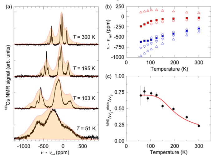
Figure 3: (a) Temperature dependence of the ^{133}\text{Cs} MAS NMR spectra ( \nu_{\text{R}} = 25 kHz) of fcc \text{Cs}_3\text{C}_{60} . The corresponding static ^{133}\text{Cs} NMR spectra (shaded areas – data taken from Ref. 4) are included for comparison. (b) Temperature dependence of the ^{133}\text{Cs} MAS NMR shifts of the components of the tetrahedral (T,
