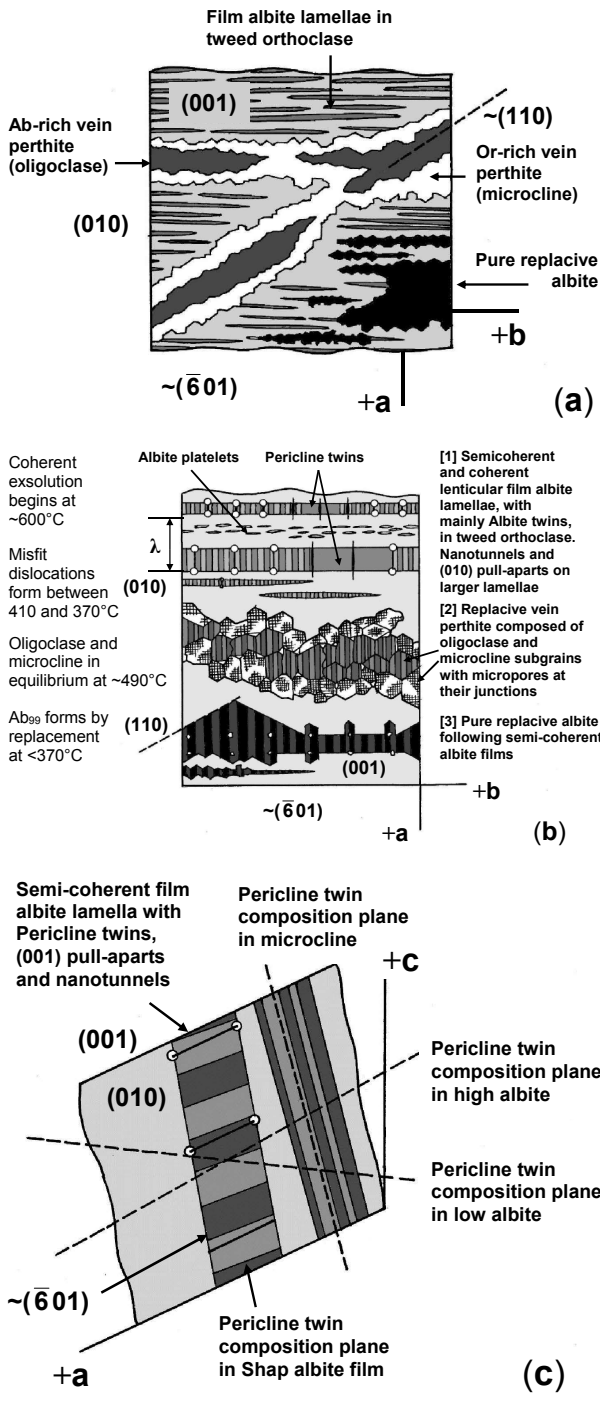
FIGURE 1. Cartoons illustrating microtextures in alkali feldspar phenocrysts in the Shap granite. See text for supporting micrographs. Each drawing shows features visible in cleavage fragments (or in similarly orientated thin sections) resting on the best-developed cleavages, (001) (a,b) and (010) (c), with outlines defined by the second cleavage and the “Murchison plane,” near (\bar{6}01) . Shades of gray approximate to composition as they appear in BSE images: Or-rich feldspar is white or pale gray, Ab-rich feldspar is black or dark gray. Shades of gray are also used to indicate Albite and Pericline twins but the twins do not differ in composition. Angular relationships are drawn accurately but considerable liberties have been taken with relative scales, which cover a very large range. (a) Features visible in a (001) thin section using LM. Film albite lamellae occur in non-turbid regions and usually have periodicities in the range 5–1 \mu\text{m} and maximum thicknesses of <0.5 \mu\text{m} . The matrix K-feldspar is usually orthoclase and is featureless. Vein perthite sheets are irregular and can be 100 \mu\text{m} thick. The veins are turbid. The K-feldspar in the veins is usually microcline, and combined Albite-Pericline twinning may be visible. In Shap the Ab-rich phase in veins is oligoclase. Pure replacive albite corresponds with turbid regions forming along, and extending from, film lamellae, at various scales. (b) Features visible in a (001) foil using TEM. [1] The periodicity ( \lambda ) of thicker film albite lamellae is typically near 1 \mu\text{m} , but thinner, shorter lamellae are often present. Platelets are only a few nanometers thick and tens of nanometers in length. Albite and Pericline twins are visible in albite lamellae. In extended lamellae the periodicity of Albite twins is typically ~20 nm but varies in proportion to the thickness of the lamellae (shown qualitatively). In Shap, Pericline twins in albite are sub-parallel to (001) (see c), and the albite appears untwinned viewed on (001). The orthoclase has visible tweed. Nanotunnels (formed by dissolution along misfit dislocations), and pull-aparts, develop on thicker film lamellae; their spacing varies with lamellar thickness. Both features can be imaged on HF etched cleavage surfaces using SEM. [2] Vein perthite is composed of parallel oligoclase and microcline subgrains, the latter concentrated near the edges of veins. Micropores form at subgrain junctions, causing optical turbidity. [3] Late replacive albite begins to form as 10 nm thick peg-shaped subgrains nucleated on nanotunnels, which grow and merge to form albite regions on >10 \mu\text{m} scales. Subgrains often have the {110} Adularia habit. Albite twin periodicities are >20 nm and micropores are abundant. (c) Orientation of features visible on (010). The drawing is at TEM scale; film lamellae are usually <1 \mu\text{m} thick. Albite film lamellae and Pericline twins in microcline are usually visible using LM but Pericline twins in albite lamellae require TEM. Nanotunnels and pull-aparts require TEM, or SEM of HF-etched surfaces. The composition plane of Pericline twins (the so-called rhombic section) in alkali feldspars rotates about the b -axis depending on composition and structural state [broken lines, from Smith and Brown (1988), Fig. 18.8]. In Shap the Pericline twins in film perthite lamellae are close to the high albite position, although they are composed of low albite (see Fitz Gerald et al. 2006). The Or-rich feldspar containing film lamellae is tweed orthoclase, with microcline occurring only in veins (b, [2]) but many K-feldspars from granites are predominantly microcline with tartan twinning on LM scales. In this case film albite lamellae in (\bar{6}01) are sub-parallel to Pericline twins in microcline and may be hard to see using LM. Difference in relief can show the presence of film lamellae. Far from crystal surfaces, nanotunnels are <10 nm in diameter, but near surfaces they are enlarged by weathering to >1 \mu\text{m} (Lee and Parsons 1995; Lee et al. 1998). Pull-aparts are in (001) and therefore make a small angle with Pericline twins.
