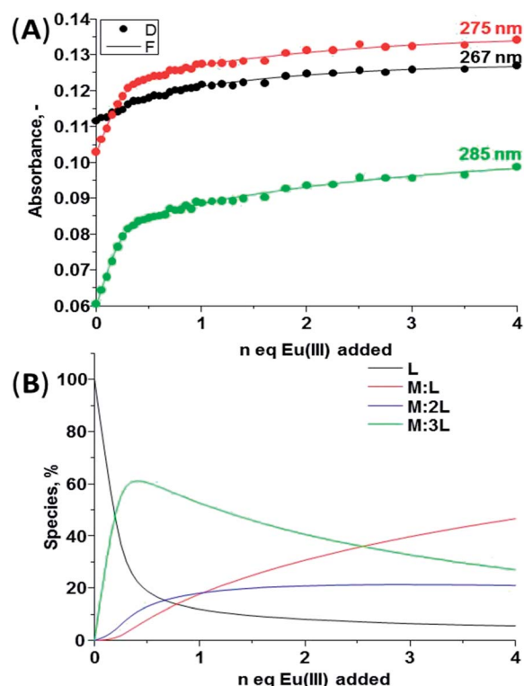
Fig. 5 (A) Experimental binding isotherms and their corresponding fit obtained using non-linear regression analysis program SPECIFIT®, (B) speciation-distribution diagram obtained from the fit of the changes in the absorption spectrum of 1(S) upon addition of Eu(CF 3 SO 3 ) 3 in CH 3 CN (25 °C, 0.05 M (C 2 H 5 ) 4 NCl).
