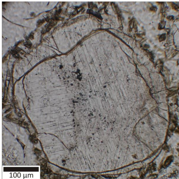
Figure 3: A quartz crystal from green impact melt rock showing three sets of decorated planar deformation features.
