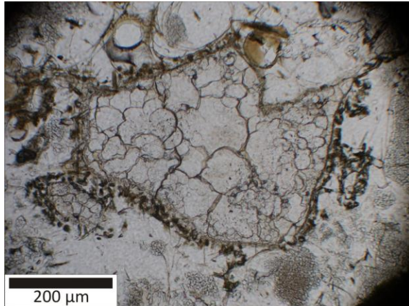
Figure 2: A quartz crystal embedded in a glassy matrix from a green impact melt rock showing ballen texture.
