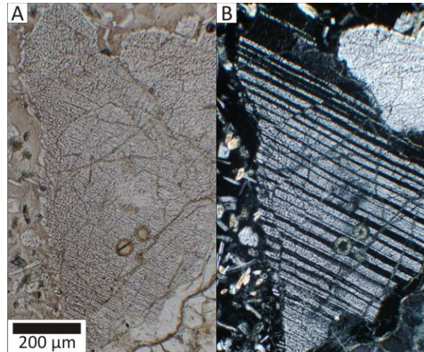
Figure 1: A grain of plagioclase feldspar from a thin section of green impact melt rock exhibiting sieve texture in plane polarized light (A), and preserved twinning in cross-polarized light (B).
