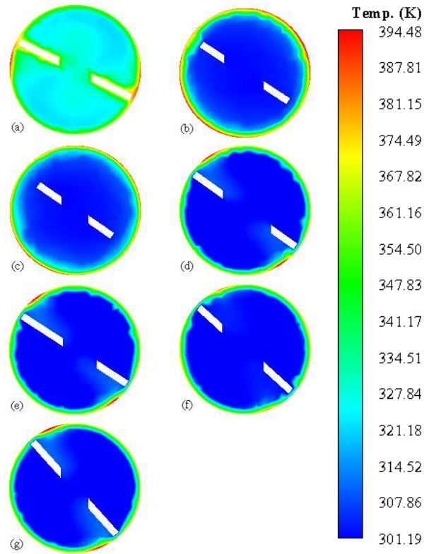
Figure 2. Contour plots of static temperature (K) for the domains of (a) TATCT, (b) TATCT w1 , (c) TATCT w2 , (d) TATCT a1 , (e) TATCT a2 , (f) TATCT y1 and (g) TATCT y2 for Re = 20000 .
