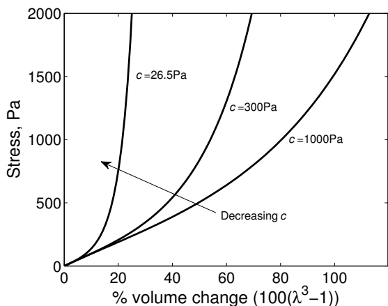
FIG. 2: Stress-strain relationships for the Fung elastic model, as given by equation (5), with bulk modulus K=380\text{Pa} , for three values of the strain stiffening parameter c . The gradient of each curve gives a measure of the stiffness: a steeper slope indicates that the mixture is more stiff, as a greater stress is required to produce a particular volume change. We observe that all these curves exhibit strain stiffening, whereby the material becomes stiffer at greater strains. However, at lower values of c , the stiffening occurs at smaller volume changes.
