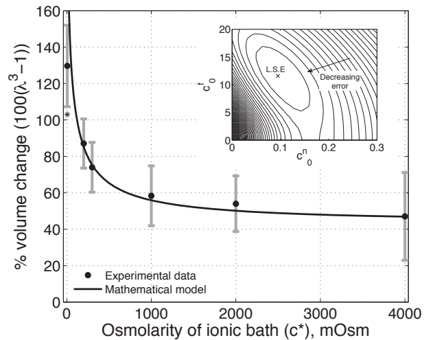
FIG. 4: Main figure: The solid curve shows solutions to (11) for the values of FCD and non-permeating solute concentrations ( c_0^f and c_0^n respectively) that minimise the mean squared error (see inset). Black circles show experimental data from [9], where the error bars signify the minimum and maximum expected range based upon the standard error of the mean. The bulk modulus is K=380\text{Pa} for all of these computations. *: the data point for the 6mOsm solution bath is excluded from the fitting, see text. Inset: Contours showing the mean squared error of solutions across a range of FCD c_0^f and fixed osmole c_0^n concentrations, compared to the experimental data shown in the main figure. Values which correspond to the least squared error (L.S.E) are c_0^f=11.6\text{mEq/l} and c_0^n=0.09\text{mOsm} .
