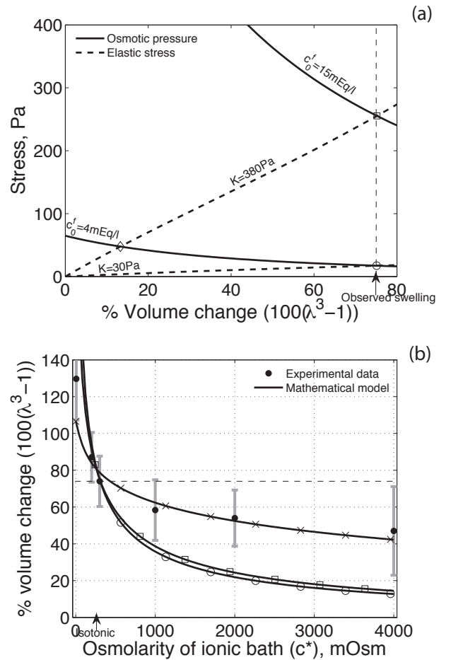
FIG. 3: (a) Elastic stress within the tissue (dashed curves) and osmotic pressure due to the Donnan effect (solid curves) in an isotonic solution ( c^* = 300\text{mOsm} ) as a function of tissue volume change. Intersections between the elastic stress and osmotic pressure give solutions to equation (9) for a particular parameter set. For an FCD of c_0^f=4\text{mEq/l} and bulk modulus K=380 we see that only 15% volume change would be expected, yet experimentally 74% was observed. Increasing the FCD to c_0^f=15\text{mEq/l} or decreasing the bulk modulus to K=30\text{Pa} allows 74% swelling. (b) Shows expected swelling (solutions to equation (9)) as a function of bath ionic concentration, for comparison with experimental data from Elkin et al. [9]. The error bars signify the minimum and maximum expected range based upon the standard error of the mean given by [9]. Each of the two parameter sets that give 74% swelling in isotonic solution are used as followed: \square : c_0^f=15\text{mEq/l} , K=380\text{Pa} . \circ : c_0^f=600\text{mEq/l} , K=30\text{Pa} . Additionally we show the curve obtained by performing a least squares fit for the bulk modulus and FCD. \times : c_0^f=157\text{mEq/l} , K=4475\text{Pa} . These parameters are unphysiological.
