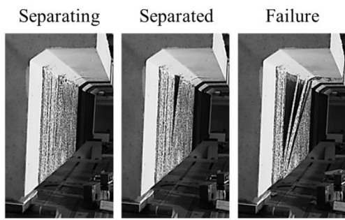
(a) Unanchored U-wrap LB1.3U
