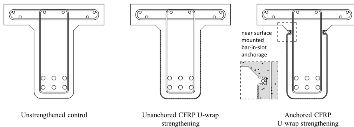
Fig. 2. CFRP strengthening arrangements
