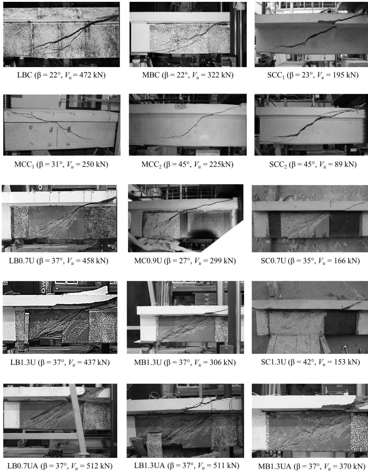
Fig. 4. Failure modes, showing critical web shear crack angles \beta and peak shear V_u .
