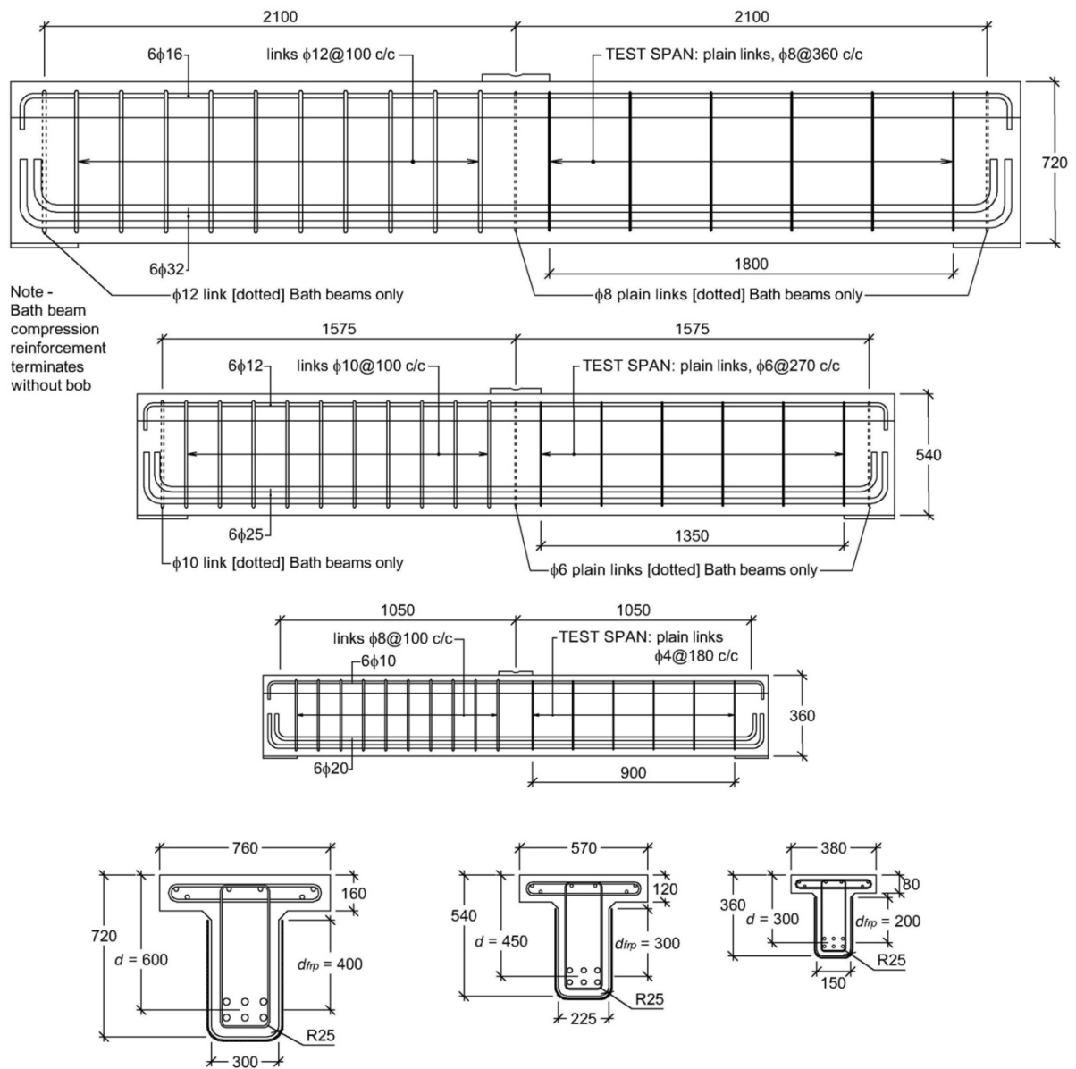
Fig. 1. Test specimens [mm]
