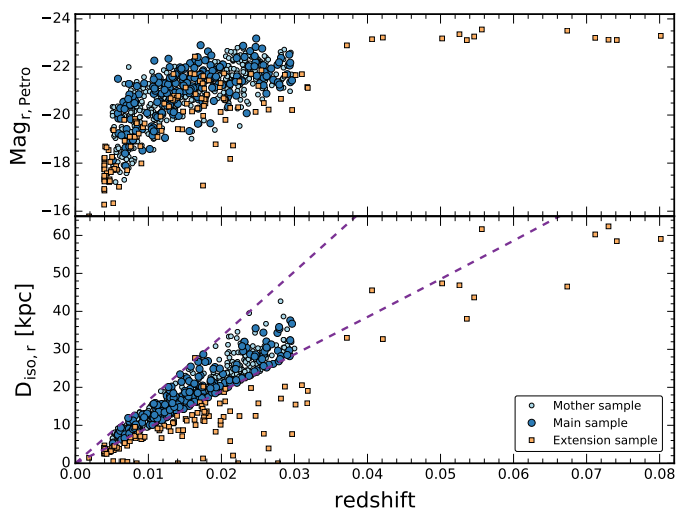
Fig. 3. The distribution of DR3 galaxies in the redshift-magnitude (up-panel) and redshift-size (lower panel) diagrams.
