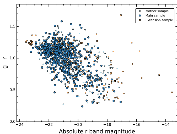
Fig. 2. The distribution of DR3 galaxies in the colour magnitude diagram.
