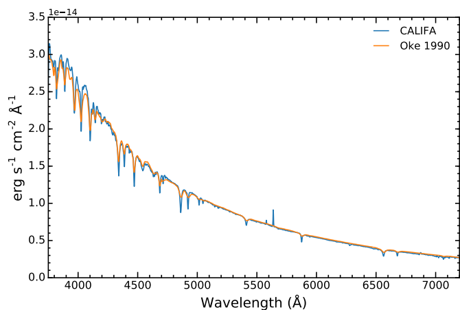
Fig. 13. Comparison between the published spectrum for the spectrophotometric standard star Hz44 and the average of the 15 spectra derived by CALIFA for the same star.
