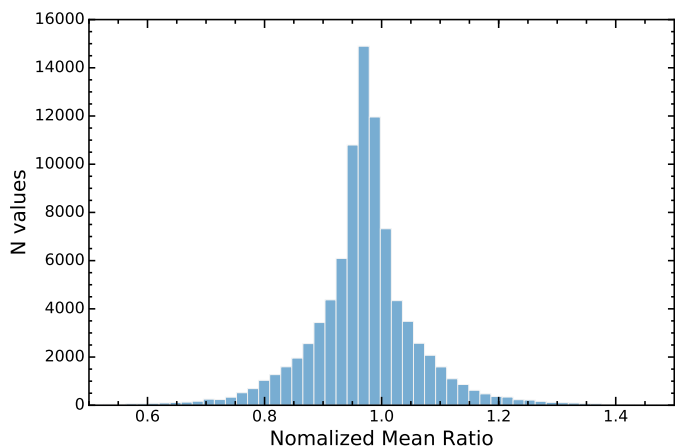
Fig. 12. Histogram of the differences between flux intensities for the published spectra for the spectrophotometric calibration stars described in Section 6.5 and the corresponding ones derived by CALIFA.
