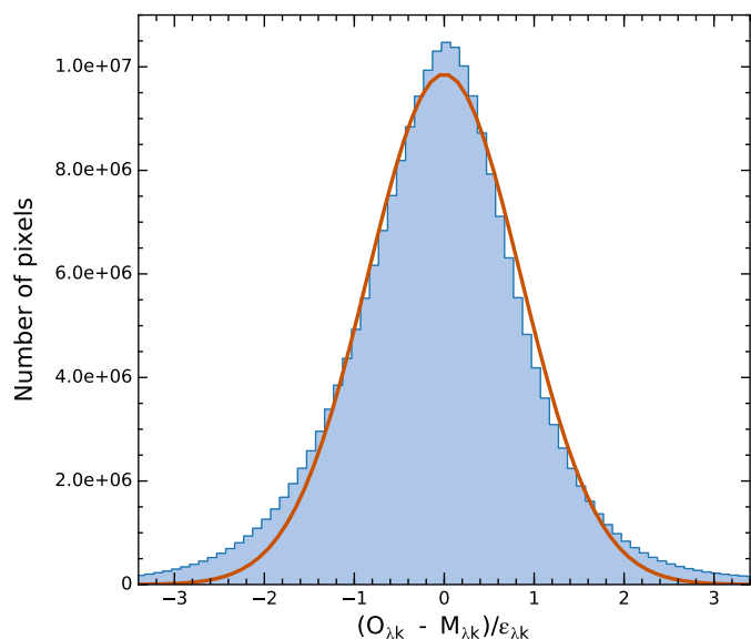
Fig. 6. Histogram of the reduced residuals (O_{\lambda,k} - M_{\lambda,k})/\epsilon_{\lambda,k} for all wavelengths, all bins ( k ) and all galaxies in DR3 (433400381 points in total). The orange line shows the best Gaussian fit to the sample.
