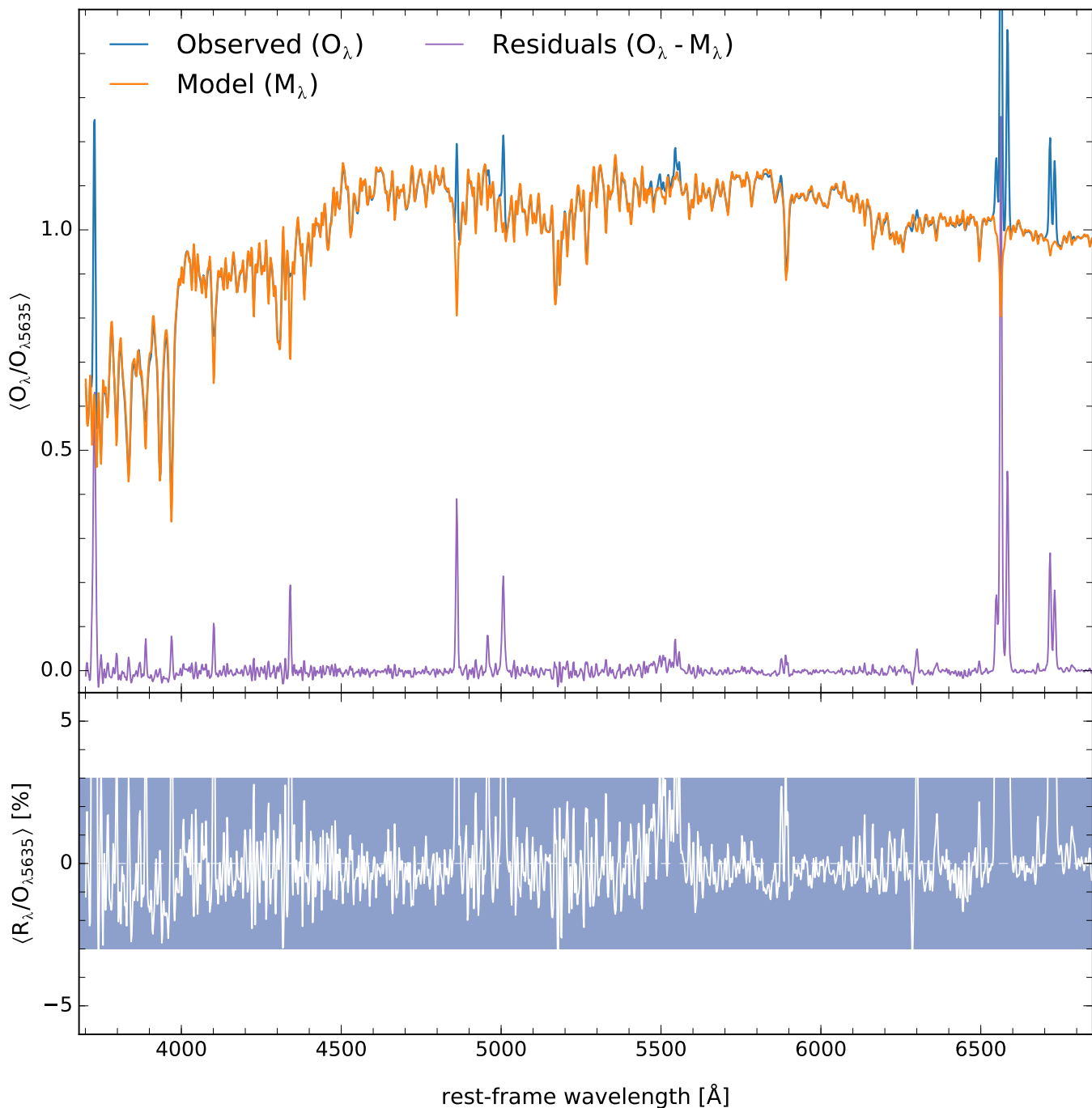
Fig. 11. Statistics of the spectral residuals Top panel: The mean normalized spectrum of 251313 bins from 446 galaxies. The mean PIPE3D fit is overlotted in orange, while the mean residual is plotted at the bottom of the panel (purple). Bottom panel: Zoom of the residual spectrum. The shaded rectangle encompasses the \pm 3\% area.
