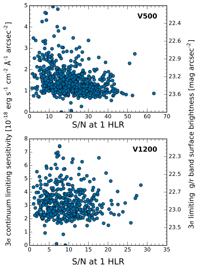
Fig. 14. Limiting 3\text{-}\sigma continuum sensitivity per spaxel and spectral resolution element as a function of the average continuum S/N at the half-light radius (HLR). The corresponding broadband surface brightness limits in r (V500) and g (V1200) are indicated on the right y-axis. The limiting continuum sensitivity and the S/N were computed from the median signal and noise in the wavelength region 4480–4520 Å and 5590–5680 Å for the V1200 and V500 data, respectively.
