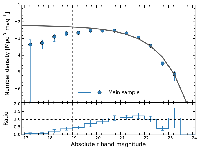
Fig. 4. Top panel: r -band luminosity functions for the SDSS reference sample from Blanton et al. (2005) (solid line) and the DR3 Main Sample. Error bars represent Poissonian uncertainties. Bottom panel: ratio between the Main Sample and SDSS.
