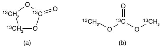
Figure 1: 13 C-enriched (a) EC and (b) DMC electrolyte molecules.
