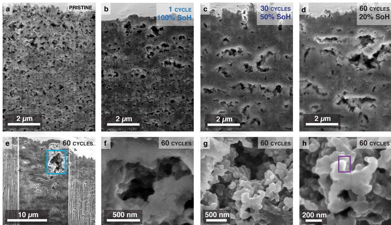
Figure 8: (a–d) SEM micro images of FIB cross sections, showing the pore structure of the electrodes after 0, 1, 30, and 60 electrochemical cycles. (e) Analysis region for (f, g, h). High magnification views of an electrode after cycle 60 (20% SoH) shows evidence of SEI growth on the C and Si particle surfaces of the electrode.
