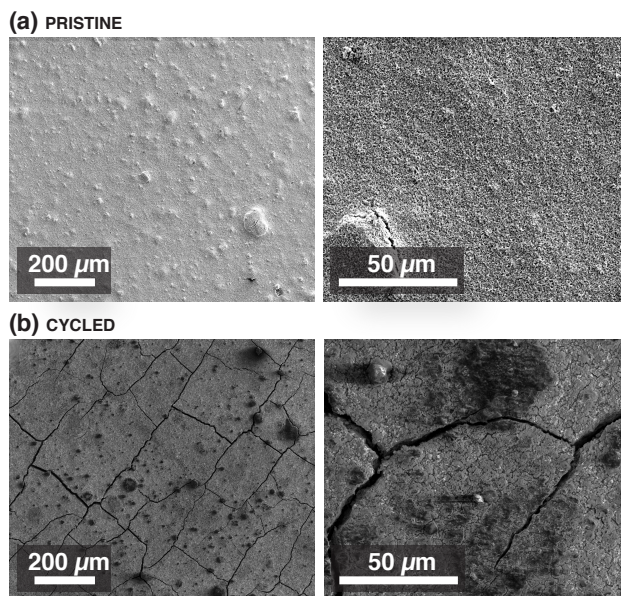
Figure 7: SEM micro images of a (a) pristine uncycled electrode and (b) cycled electrode sample, after 60 electrochemical cycles.
