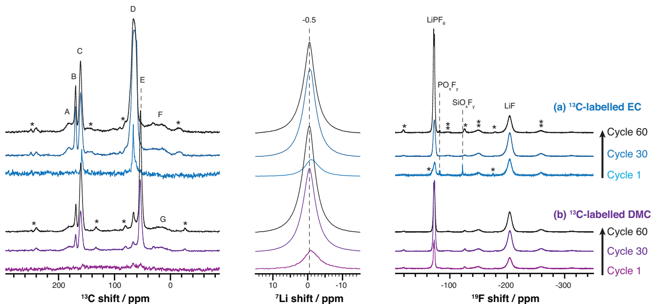
Figure 4: Direct excitation ^{13}\text{C} , ^7\text{Li} , and ^{19}\text{F} ssNMR experiments of electrode samples prepared with (a) ^{13}\text{C} EC (blue) and (b) ^{13}\text{C} DMC (purple) labelled electrolytes. Measurements were performed on electrode samples from coin cells cycled through 1, 30, and 60 electrochemical cycles (approximately 100, 50, 20% SoH). Single pulse ^{13}\text{C} and Hahn echo ^{19}\text{F} spectra were acquired on a 500 MHz spectrometer with 10 kHz and 25 kHz MAS rate, respectively. ^7\text{Li} single pulse spectra were acquired on a 400 MHz spectrometer with 30 kHz MAS rate. ^{13}\text{C} peak assignments A–G are summarized in Table 1. Asterisks indicate spinning sidebands.
