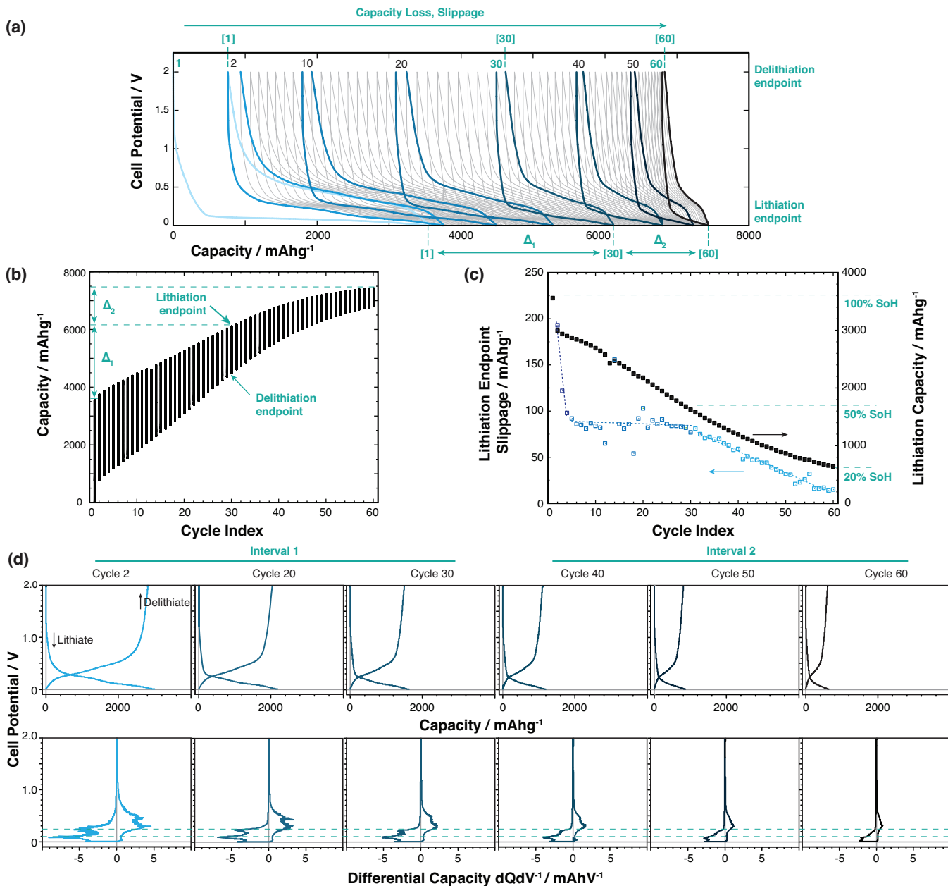
Figure 2: Electrochemical cycling of a Si/C/CMC composite electrode cycled against Li metal and plotted by (a) cell potential vs. capacity and (b) capacity vs. cycle index 1–60. In (c) the slippage (axis left, unfilled points) is compared to the lithiation/discharge capacity (axis right, filled points) for each cycle index. The slippage is approximated by three regions, indicated by linear fits. The lithiation endpoint slippage is defined as the difference of the lithiation endpoints for incremental cycles and is a measure of irreversibly consumed Li + in the system per cycle. \Delta_1 and \Delta_2 indicate the total irreversible capacity between cycles 1–30 and 30–60, respectively. In (d) selected capacity and differential capacity dQdV^{-1} curves for cycle 2–60 are presented, showing the detail of the lithiation/delithiation processes of the Si electrochemistry. Cycles 2–30 and 30–60 are labelled interval 1 and 2, respectively. Dashed lines indicate the initial potential of the electrochemical lithiation processes, occurring at approximately 250 and 100 mV.
