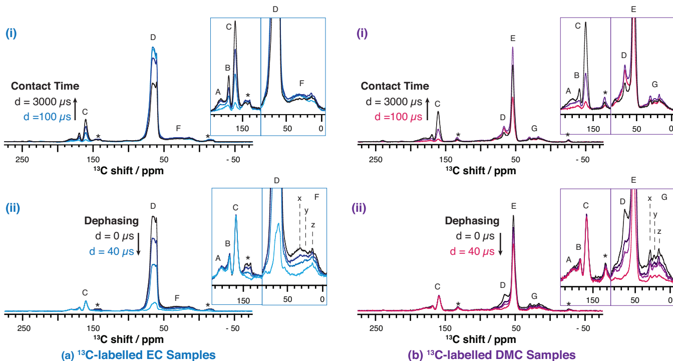
Figure 6: ssNMR ^1\text{H} - ^{13}\text{C} cross polarization and dephasing experiments of electrode samples prepared with (a, left) ^{13}\text{C} EC and (b, right) ^{13}\text{C} DMC labelled electrolytes. When delay times are varied in the experiment, different C functional groups can be identified based on their attenuation rates. In (a-i, b-i) CP contact times in the experiments were varied and in (ii-a, ii-b) dephasing times were varied. See Supporting Information for ssNMR pulse sequence details. Increasing CP contact times of (a-i) 100, 500, 1000, 3000 \mu\text{s} and (b-i) 100, 500, 3000 \mu\text{s} correlate with increasing carbonate and carboxyl signal intensities. Using a fixed CP contact time of 500 \mu\text{s} , increasing dephasing times of (a-ii) 0, 10, 15, 40 \mu\text{s} and (b-ii) 0, 15, 20, 30 \mu\text{s} correlate with decreasing signal intensities of proton-bonded carbons. Asterisks indicate spinning sidebands.
