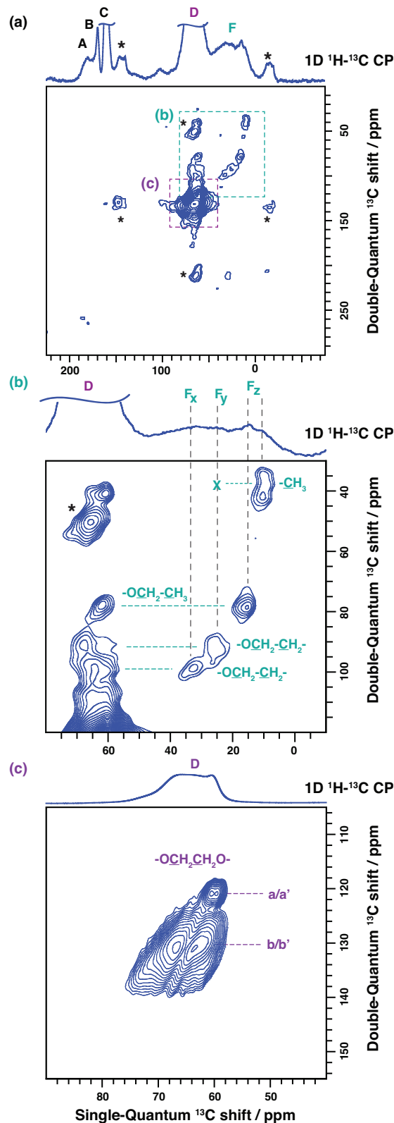
Figure 5: ^{13}\text{C} DQ/SQ homonuclear correlation ssNMR experiment performed on the 30 cycle sample prepared with ^{13}\text{C} -labelled EC electrolyte. The correlations in the J-based ^1\text{H} - ^{13}\text{C} CP refocused INADEQUATE experiment show the pairs of resonances which are bonded. See Supporting Information for views of the spectra with lower contour levels. Asterisks indicate spinning sidebands.
