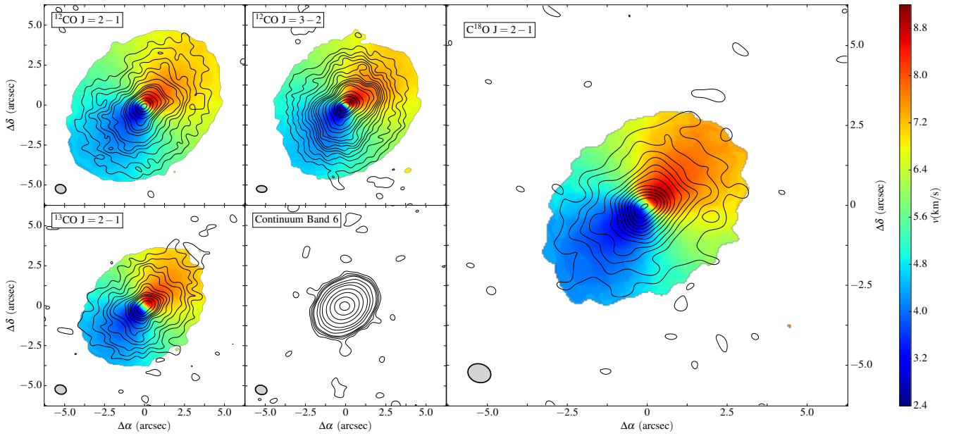
Figure 1. Integrated line emission (contours) and intensity weighted velocity (colour) maps of 12 CO J=2-1, 12 CO J=3-2, 13 CO J=2-1, C 18 O J=2-1 and continuum map of Band 6. The contours are levels of (2, 4, 6, 8, ...) \times \sigma noise. The innermost contour has the following levels: \sim 100 \times \sigma ( 12 CO J=2-1), \sim 100 \times \sigma ( 12 CO J=3-2), \sim 28 \times \sigma ( 13 CO J=2-1), \sim 52 \times \sigma (C 18 O J=2-1) and \sim 796 \times \sigma (continuum). The velocity maps discard the data at a level \lesssim 5 \times \sigma noise. The respective \sigma are given in Table 2. The synthesized beam is plotted in the bottom left corner of each panel.
