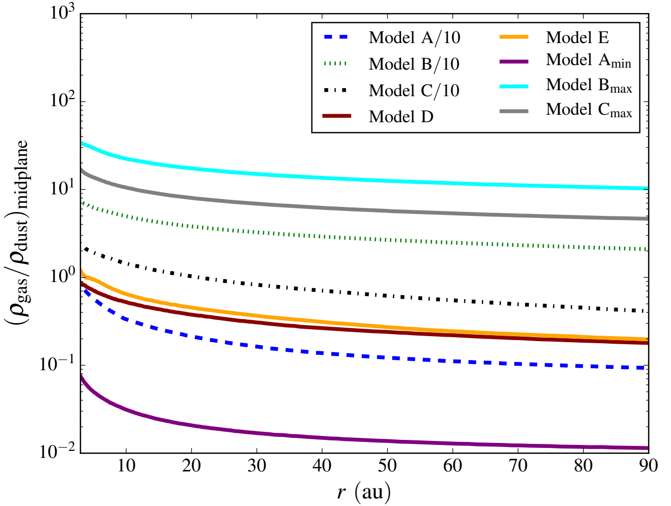
Figure 10. Gas to dust mass ratio in the disc midplane for our models (A-C)/10, D, E, A min , B max and C max in the inner disc regions ( R < 90 au).
