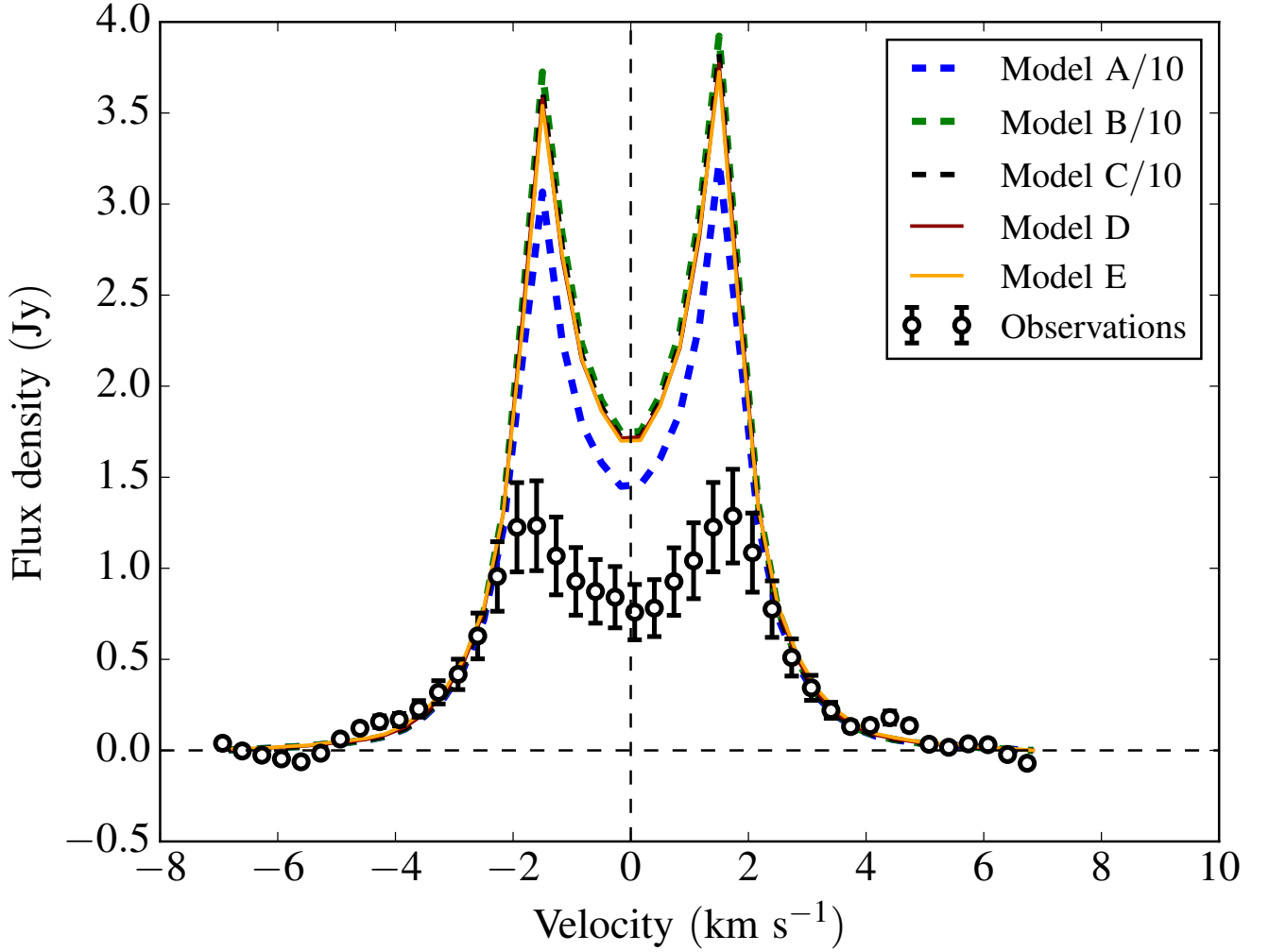
Figure 8. C^{18}O line profile for the whole disc for our 5 fiducial models (colours) and as observed (dots, error bars represent a 10% flux calibrations uncertainty, Guidi et al. (2016)). The profiles were centred around a velocity of 0 \text{ km s}^{-1} . All models from the same series (that have C^{18}O abundances in the allowed range) have the same line profile (as they have different C^{18}O abundances and gas masses, but the same C^{18}O mass). Our models match the emission from the inner disc regions (wings of the line profile) very well, whereas they over predict the emission in the outer disc regions (peaks of the spectrum). Our modelling approach is however best suited for the inner disc regions.
