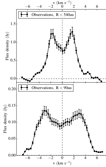
Figure 5. \text{C}^{18}\text{O} J=2-1 line profile (ALMA observations) using the emission from the whole disc (upper panel) and from within the 90 au snowline radius. The error bars represent a 10% flux calibration uncertainty (Guidi et al. 2016). We centred the spectra on 0 \text{ km s}^{-1} . The systemic velocity is v_{\text{sys}}=5.8 \text{ km s}^{-1} .
