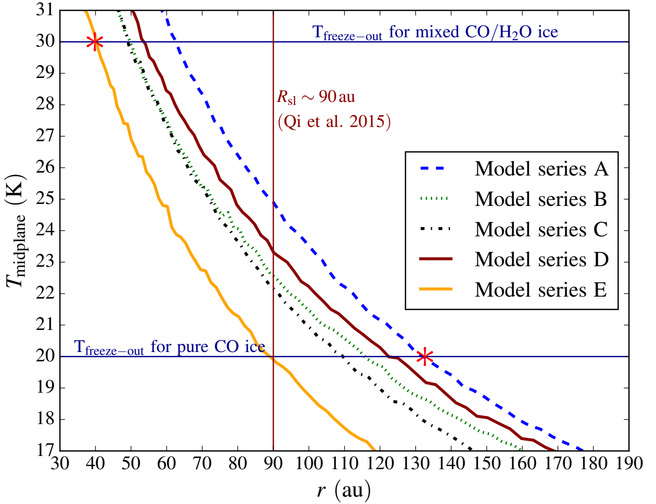
Figure 4. Midplane temperature as a function of radius for our 15 disc models that match the observed SED. Models from the same series have exactly the same midplane temperature structure (see Section 3.1.1). In dark red (vertical) we plot the observed snowline radius \approx 90 au (Qi et al. 2015). The upper and lower limits of the freeze-out temperature ( \sim 20 - 30 K) as found by e.g. Collings et al. (2004) are plotted as horizontal lines. The red asterisks indicate where the snowline location could be between \sim 40 and 135 au due to a plausible range of freeze-out temperatures of 20-30 K if the snowline location was not known unambiguously from observations.
