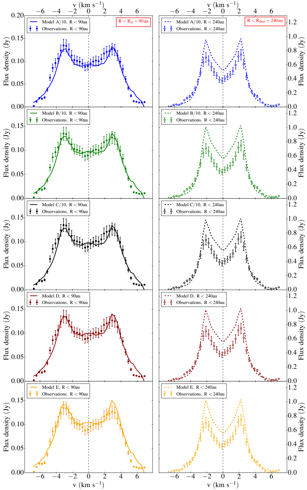
Figure 7. \text{C}^{18}\text{O} J=2-1 line profiles for our 5 models: We show the emission from within the CO snowline radius (90 au) as well as from a disc region with R < 240 au (this corresponds to the outer disc radius as obtained from mm continuum observations). The line profiles from our models are given by the lines (solid for R = 90 au, dashed for R = 240 au), the spectra of the observations by the respective dots. The error bars reflect the 10% flux calibration uncertainty of the observations. All models of the same series that have abundances in the range of \text{C}^{18}\text{O} abundances we consider will have the same flux densities because the \text{C}^{18}\text{O} masses and temperature structures are the same for each of these model series. The profiles were centred around 0 \text{ km s}^{-1} (the systemic velocity is v_{\text{sys}} = 5.8 \text{ km s}^{-1} ).
