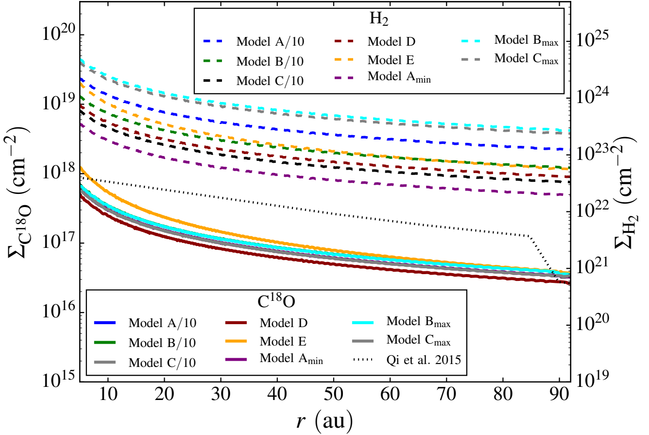
Figure 9. Left y-axis: Column number density of C^{18}O for our models (A-C)/10, D, E, A_{\min} , B_{\max} and C_{\max} for regions within the 90 au snowline radius, given by the solid colourful lines. We overplot the one obtained by Qi et al. (2015) (dotted black line, extrapolated from 50 au inwards). Right y-axis: Corresponding column density of H_2 , given by the dashed lines for the individual models. The masses of both C^{18}O and H_2 that correspond to these column densities are given in Table 6.
