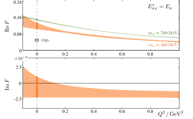
FIG. 13: The real and imaginary parts of the form factor determined in this work evaluated at the \rho pole (orange). For comparison we show the form factor obtained in Ref. [46] for a heavier quark mass, where the \rho is stable (green). Also shown is the experimentally determined value for the \rho\pi photocoupling [62, 63].
