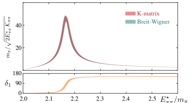
FIG. 7: Top panel shows m_\pi/\sqrt{2E_{\pi\pi}^* \mathcal{K}_{\pi\pi}} as a function of the \pi\pi energy, as defined in Eq. (22). The two parameterizations of the phase-shift given in Eqs. 14 and 15 are consistent and feature the expected enhancement of the transition amplitude in the vicinity of the \rho . Lower panel shows the \pi\pi scattering phase shift for comparison.
