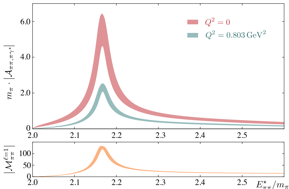
FIG. 14: m_\pi |\mathcal{A}_{\pi\pi, \pi\gamma^*}| for two values of Q^2 as a function of E_{\pi\pi}^* along with the elastic \pi\pi P -wave scattering amplitude.
