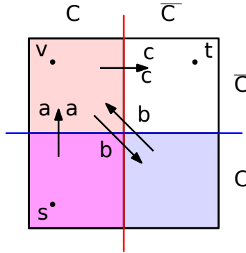
Fig. 3. Diagram for the proof of Lemma 5.2. Here the labels indicate the net flow between two sets under flows f and f' .
