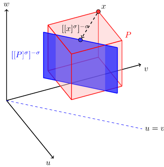
Fig. 2. Folding and unfolding a polytope P \subseteq \mathbb{Q}^{\{u,v,w\}} with respect to \sigma = \{u \rightarrow 0, v \rightarrow 0, w \rightarrow 1\} .
