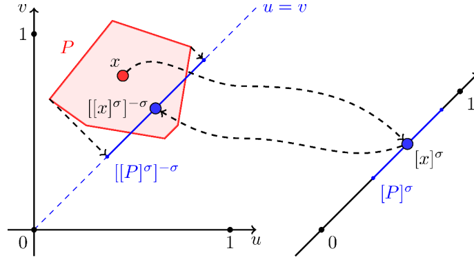
Fig. 1. Folding and unfolding a polytope P \subseteq \mathbb{Q}^{\{u,v\}} with respect to \sigma = \{u \rightarrow 0, v \rightarrow 0\} .
