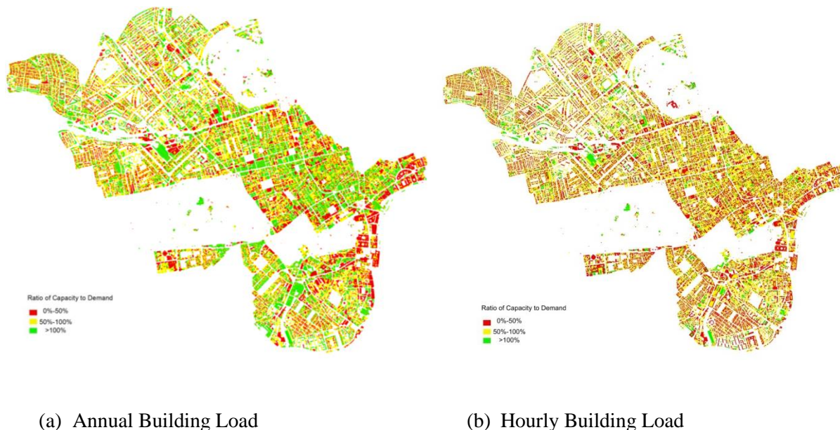
Figure 5 Spatial Distributions of C/D Ratio with Various Building Load Estimation Methods under Scenario 1
