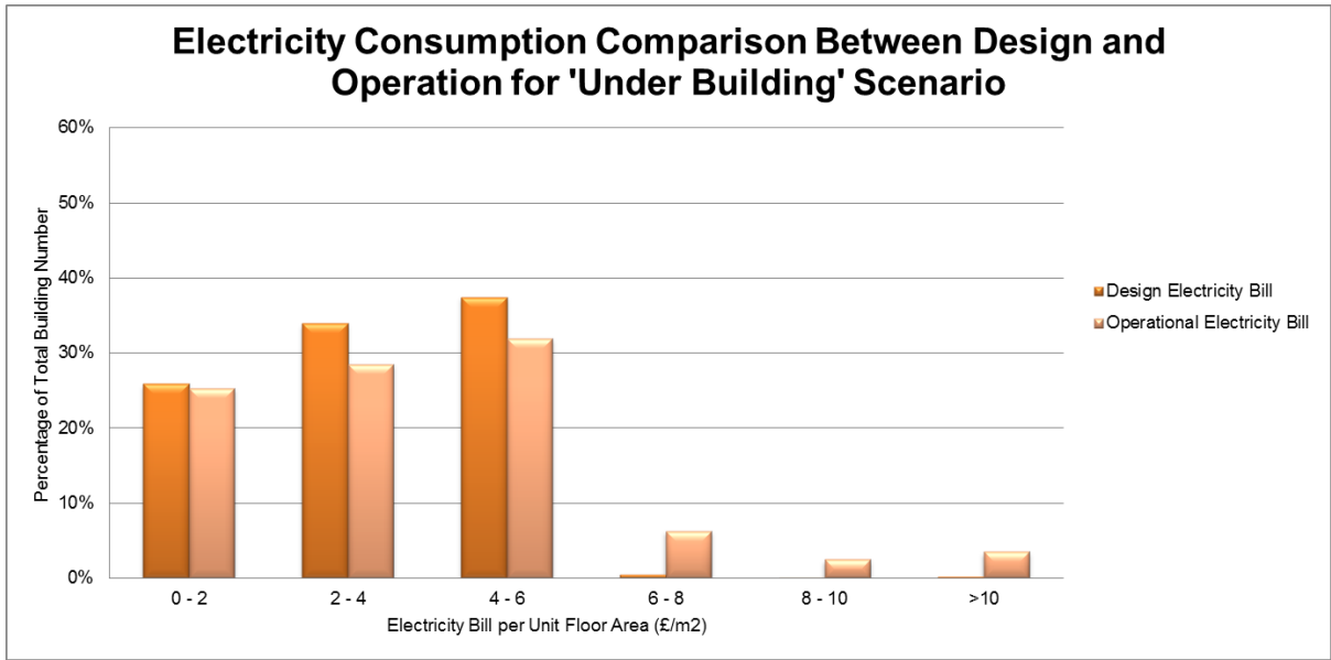
Figure 8 Electricity Consumption Comparison between Design and Operation under Scenario 1
