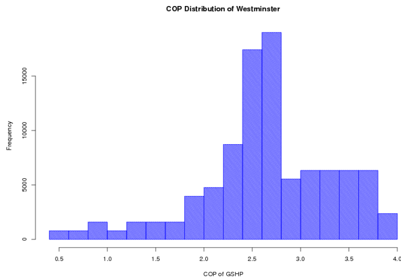
Figure 1 COP Frequency Distribution under Operation for All the buildings in Westminster
