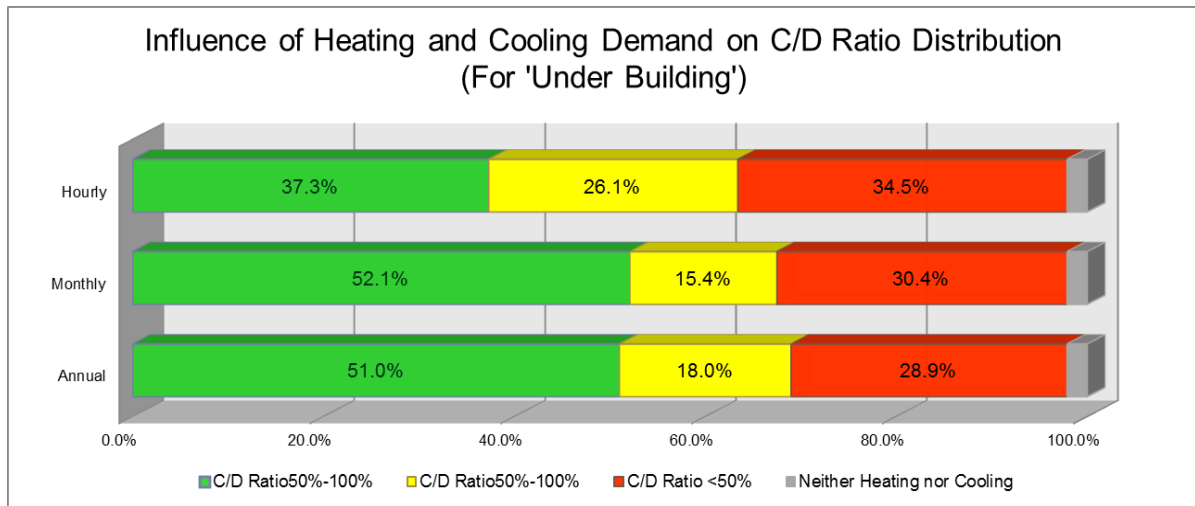
Figure 4 C/D Ratio Frequency Distributions with Various Building Load Estimation Methods under Scenario 1
