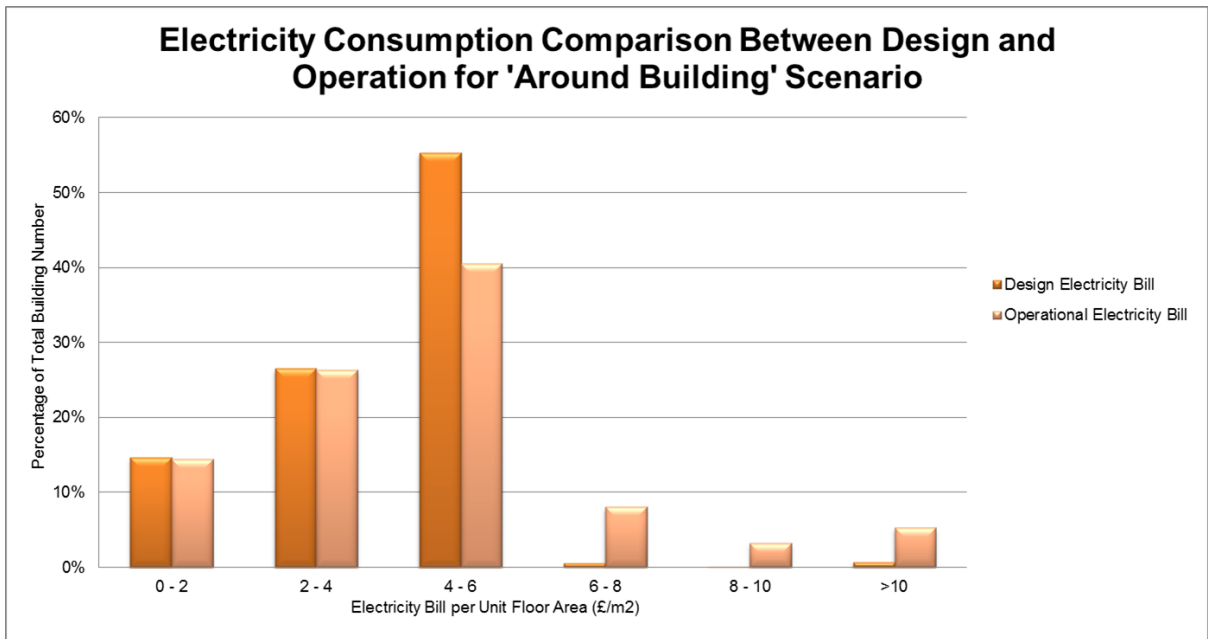
Figure 10 Electricity Consumption Comparison between Design and Operation under Scenario 2
