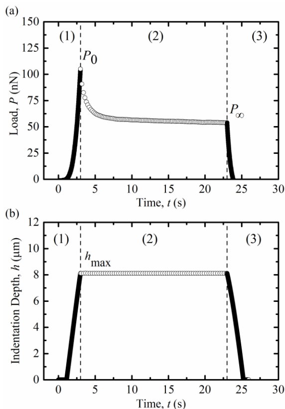
Fig. 1 Representative (a) load vs. time ( P-t ) data and (b) indentation depth vs. time ( h-t ) data for a 100 nN indentation load. Initially, P and h are increased to P_0 and h_{max} , respectively (region 1). On reaching the maximum load, P_0 , indentation depth is maintained for a 20 s hold period while P relaxes to P_\infty (region 2). After the hold period, the AFM probe is retracted from the surface (region 3).
