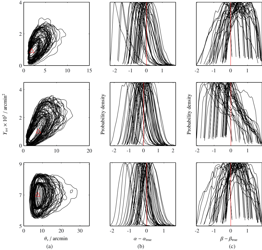
Fig. 31. Posterior distributions for simulated clusters with realistic noise levels (see text for details), and varying GNFW shape parameter values based on the REXCESS sample (Böhringer et al. 2007; Arnaud et al. 2010). a) shows the two-dimensional \theta_s and Y_{\text{tot}} posterior, and b) and c) show the one-dimensional posteriors for \alpha and \beta , shifted to be centred on the appropriate true value. In all cases \gamma is fixed to the universal value, \alpha has a truncated Gaussian prior based on the REXCESS sample, \beta is varied uniformly between 4.5 and 6.5, a Planck -like Gaussian prior is used on Y_{\text{tot}} and \theta_s has the conditional prior drawn from the two-dimensional prior. Results for three different angular sizes are shown (from top to bottom, \theta_s = 1.8, 4.5 and 7.4 ); the input parameter values are marked with red triangles and lines.
