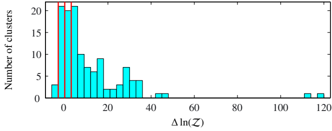
Fig. 3. Distribution of evidence ratio values in the SZ sample, with the division into detection categories given in Table 3 indicated by red vertical lines.
