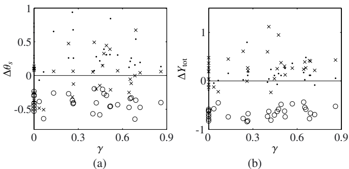
Fig. 30. Fractional difference [(\text{MAP value} - \text{true value})/(\text{true value})] in \theta_s a) and Y_{\text{tot}} b) as a function of the input value of \gamma . Clusters with \theta_s = 1.8 are plotted as dots, \theta_s = 4.5 as crosses and \theta_s = 7.4 as open circles.
