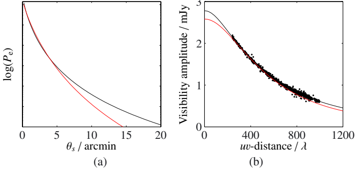
Fig. 24. A profile generated with \beta = 5.4905 , \theta_s = 1.8 (the universal profile, black lines) can be mimicked for \beta = 8.9 using \theta_s = 4.1 and adjusting Y_{\text{tot}} downward (red lines). The two profiles are almost identical over the AMI-SA range of baselines, while Planck would measure the zero-spacing flux which differs by \approx 7\% between the two models. a) Shows the pressure profiles in radial coordinates (note that the y -axis scale is log); and b) shows the profiles in uv -space for channel 5, with the simulated AMI data shown as dots. Note that this simulation has been generated with an unrealistically small amount of thermal noise.
