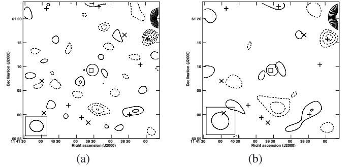
Fig. 14. SA source-subtracted map of PSZ1 G137.56+53.88 with a) natural weighting and b) a uv -taper. The rms noise levels are 109 and 150 \mu\text{Jy beam}^{-1} respectively. See Sect. 4.4 for more details on the plots.
