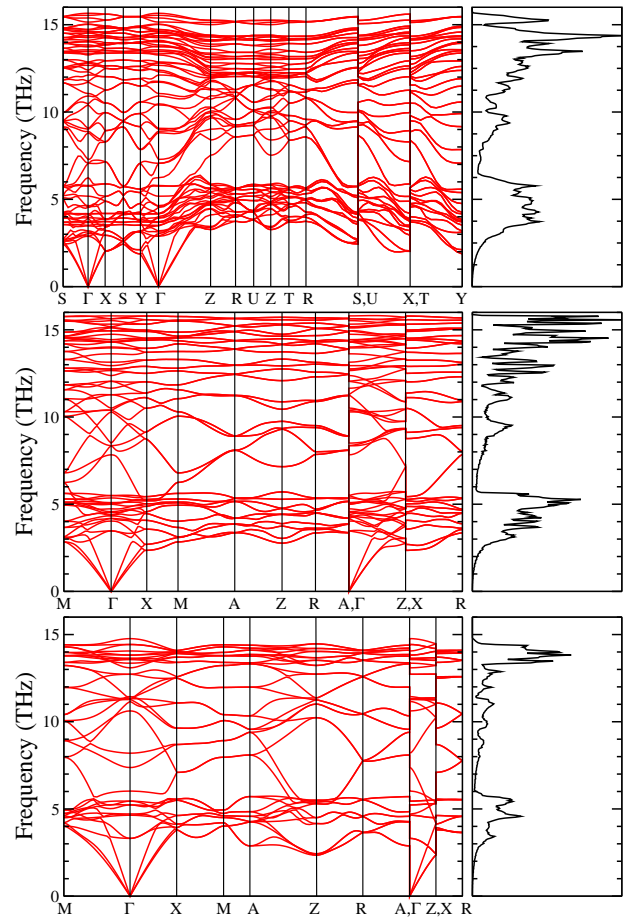
FIG. 9. (Color online) Calculated phonon dispersion relations of the Pbam, P4 1 2 1 2, and P4 2 /ncm structures of Si at zero pressure. The panel on the right of each plot shows the total phonon density of states.
