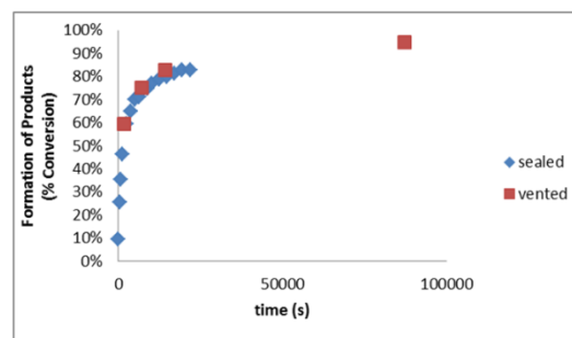
Figure 7 Comparison of overall rate of formation of aminosilanes 2a and 2b in the reaction of \text{Et}_2\text{NH} with \text{PhSiH}_3 using 10 mol % A at 70^\circ\text{C} in toluene, vented (to allow the \text{H}_2 generated to escape) and unvented (in a sealed NMR tube).
