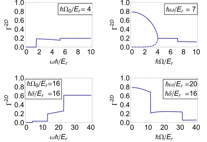
FIG. 6. (Color online) Dimensionless scattering rate \Gamma^{2D} , see Equation (59) for an initial state with particles in the lower band with momentum k = \pm|k_0| and relative momentum k_y = 0 getting inelastically scattered for the extension to a 2D setting with free motion in a transverse direction. In the top row for no detuning \hbar\delta/E_r = 0 as a function of \omega\hbar/E_r for fixed \hbar\Omega/E_r = 4 to the left and as a function of \hbar\Omega/E_r for fixed \omega\hbar/E_r = 7 to the right (dashed k = +|k_0| , full k = -|k_0| ) and at the bottom for \hbar\delta/E_r = 16 as a function of \omega\hbar/E_r for fixed \hbar\Omega/E_r = 16 to the left and as a function of \hbar\Omega/E_r for fixed \omega\hbar/E_r = 20 to the right as indicated in Fig. 4. The rate shows jumps at the opening/closing of scattering channels corresponding to the borders in Fig. 4.
