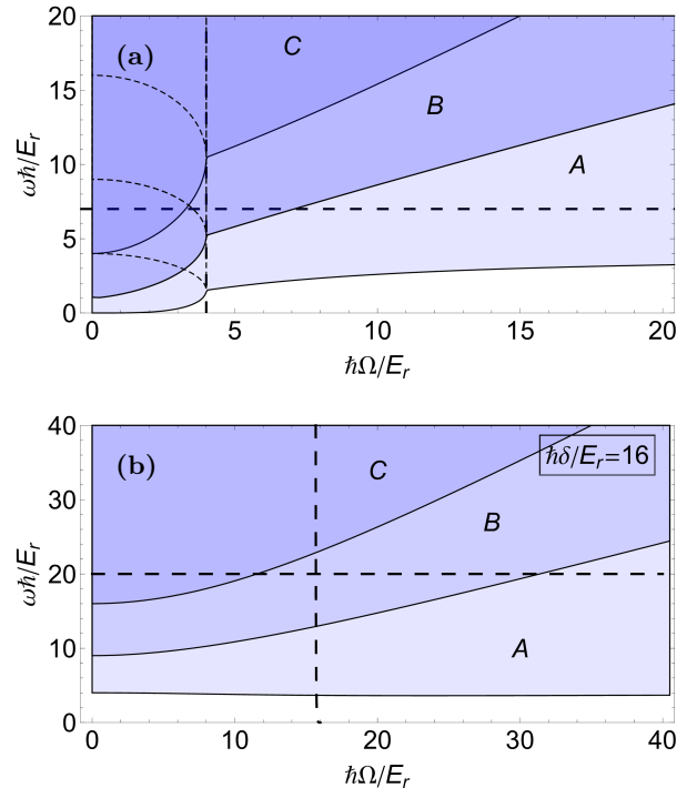
FIG. 4. (Color online) Stability diagram for (a) \hbar\delta/E_r = 0 and (b) \hbar\delta/E_r = 16 with initial state of two particles with quasi-momentum k = k_0 in lower band. For no detuning and \hbar\Omega/E_r < 4 both cases of k = +|k_0| (dashed lines) and k = -|k_0| (full lines) are shown, with detuning the minimum is unique. Shaded regions correspond to parameter regimes in which inelastic scattering is allowed. The bottom region (A) in light blue corresponds to inelastic scattering where both particles remain in the lower bands, i.e. the (-, -) -final state, in the middle region (B) particles can scatter either into the (-, -) or the (+, -) -final state and in the top region (C) scattering into all states (-, -) , (+, -) and (+, +) is allowed. The thick dashed lines of constant \omega\hbar/E_r and of constant \Omega\hbar/E_r correspond to the cuts along which the scattering rate is shown in Fig. 5 and Fig. 6.
