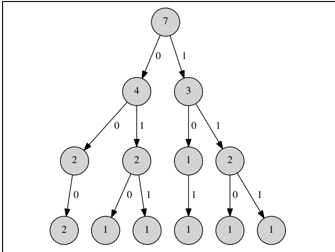
Figure 1: The binary tree representing the multiset: \{000, 000, 010, 011, 101, 110, 111\} . The count at each node indicates the number of strings starting with the node’s prefix: e.g. there are 7 strings starting with the empty string, 4 strings starting with 0, 3 strings starting with 1, and 2 strings starting with 01.
