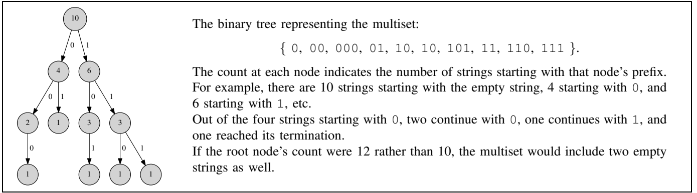
Figure 4: Binary tree representing a multiset of ten binary sequences. This tree follows the same basic structure as the tree in Figure 1, but admits sequences of variable length. The tree representation is unique for each multiset.
