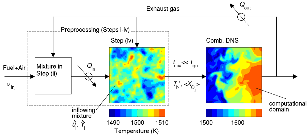
Figure 2. Schematic illustration of the two-stage approach employed for the present MILD combustion DNS. Left box: mixing DNS domain. Right box: combustion DNS domain. Steps i-iv noted in the left box are described in section 2.3
