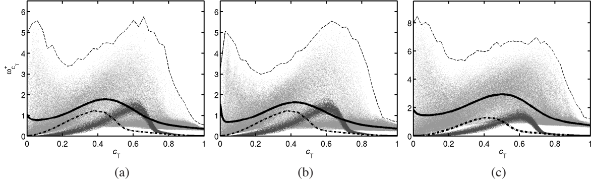
Figure 13. Variation of \omega_{c_T}^+ with c_T in (a) Case A1, (b) Case A2, and (c) Case B1. The scatter with light grey points is for MILD combustion and the dark grey points are for premixed case. The points are taken at t = 1.5\tau_D , and the thin dashed line is the maximum value observed in the DNS from the entire sampling period. Solid line: the conditional average \langle \omega_{c_T}^+ | c_T \rangle , and dash-dotted line: the respective MIFE.
