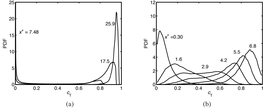
Figure 7. Typical PDF of reaction progress variable based on temperature at various x^+ locations for (a) Case C and (b) Case B1.
