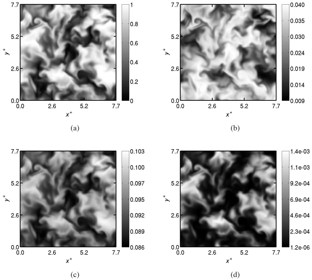
Figure 4. Typical spatial variation of preprocessed fields of (a) \hat{c}_Y , (b) \hat{Y}_{O_2} , (c) \hat{Y}_{H_2O} , and (d) \hat{Y}_{OH} in mid x - y plane obtained in Step (iv) for Case B1.
