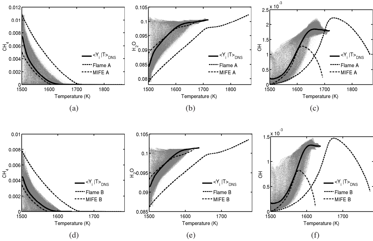
Figure 12. Variation of species mass fractions, \text{CH}_4 (a, d), \text{H}_2\text{O} (b, e), and \text{OH} (c, f) with temperature in the MILD combustion DNS (scatter), Case A1 (a–c) and Case B1 (d–f). Continuous line: the conditional average \langle Y_i | T \rangle_{\text{DNS}} of the DNS results, dashed line: the respective laminar Flames in table 1, and dash-dotted line: the respective MIFE in table 1. The data for scatter plot is taken at t = 1.5\tau_D and conditional average is calculated using data from the entire sampling period.
