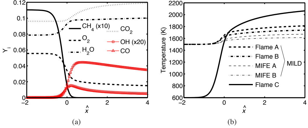
Figure 5. Variations of (a) mass fraction variations of \text{CH}_4 , \text{O}_2 , \text{H}_2\text{O} , \text{CO}_2 , \text{OH} and \text{CO} in Flame A and (b) temperature in one-dimensional laminar flames used for the MILD and premixed combustion cases.
