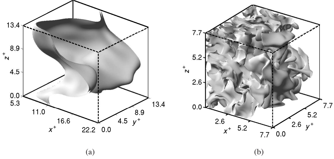
Figure 8. Typical iso-surface of reaction rate at t = 1.5\tau_D . (a) \omega_{c_T}^+ = 1.0 for the premixed case and (b) \omega_{c_T}^+ = 2.0 for Case B1. Note that only 5.3 \leq x^+ \leq 22.2 of the computational domain is shown for Case C in (a).
