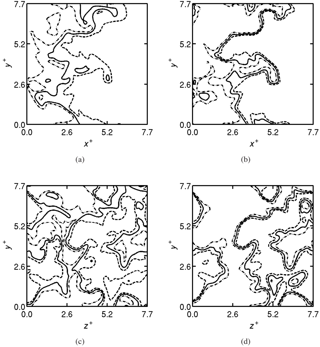
Figure 11. Typical spatial variations of the normalised temperature, T^* , (shown in a and c) and Y_{\text{OH}}^* (b and d) for Case B1. The contours are shown for the mid x - y plane (a and b), and y - z plane at x = L_x/3 (c and d) at t = 1.5\tau_D . The contour levels are 0.2 (dash-dotted line), 0.4 (continuous lines), and 0.6 (dashed lines).
