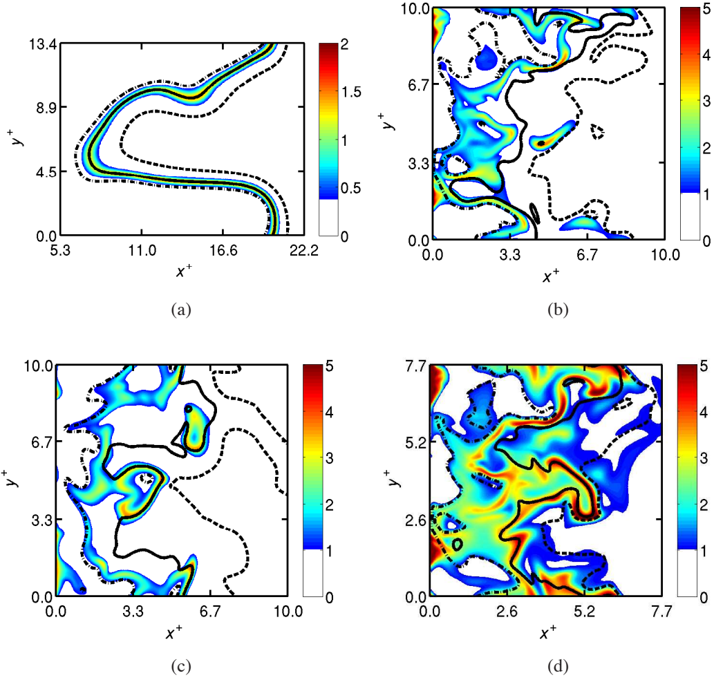
Figure 9. Variations of \omega_{c_T}^+ (colour) and c_T (lines) in the mid x - y planes for (a) Case C, (b) Case A1, (c) Case A2, and (d) Case B1. Dash-dotted line: c_T = 0.2 , solid line: c_T = 0.6 , and dashed line: c_T = 0.8 . Note that only 5.3 \leq x^+ \leq 22.2 of the computational domain is shown for Case C in (a). Snapshots are taken at t = 1.5\tau_D .
