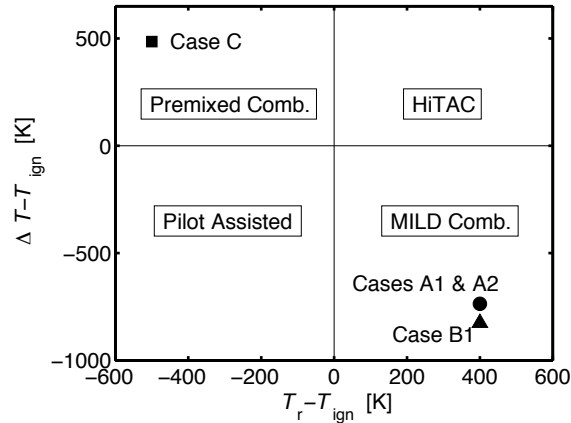
Figure 1. A diagram showing combustion types and combustion conditions considered in the present study (Cavaliere & de Joannon, 2004).
