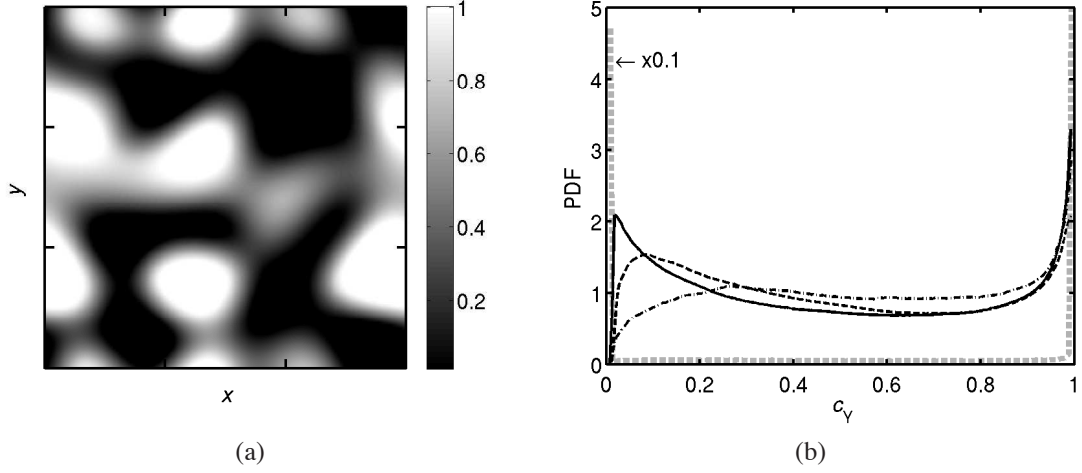
Figure 3. (a) Typical spatial variation of \hat{c}_Y field obtained in Step (iii), the field is shown for mid x - y plane. (b) Typical PDF of \hat{c}_Y in the field obtained during the preprocessing. Grey dashed line: initial field obtained in Step (iii), black solid line: preprocessed field obtained in Step (iv) to be used for Case A1, black dashed line: for Case A2, and black dash-dotted line: for Case B1.
