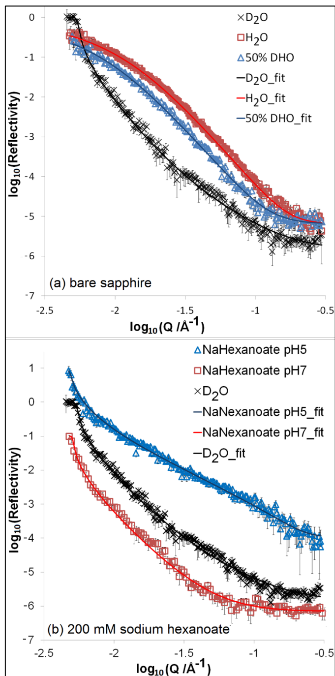
Figure 5. Neutron reflectivity of (a) the clean and bare sapphire substrate with 3 water contrasts and (b) 200 mM of sodium hexanoate at pH 5 and 7 in D 2 O on sapphire. The fits to
