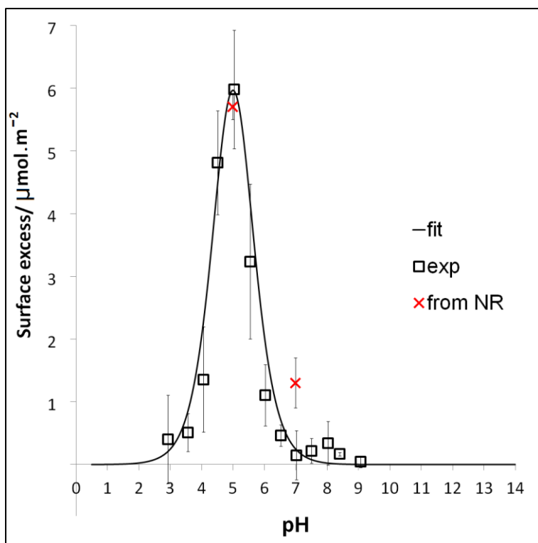
Figure 4. Surface excess of sodium hexanoate (6 mM of sodium hexanoate in 40 ml solution with 0.11 g \alpha -alumina) as a function of pH, measured by solution depletion. Fits (solid line) using the equilibrium and binding constants listed in Table 3. Two surface excess values calculated from the neutron data at pH 5 and 7 in Figure 5 and Table 2, are also included. (2-column fitting, colours for both web and paper)
