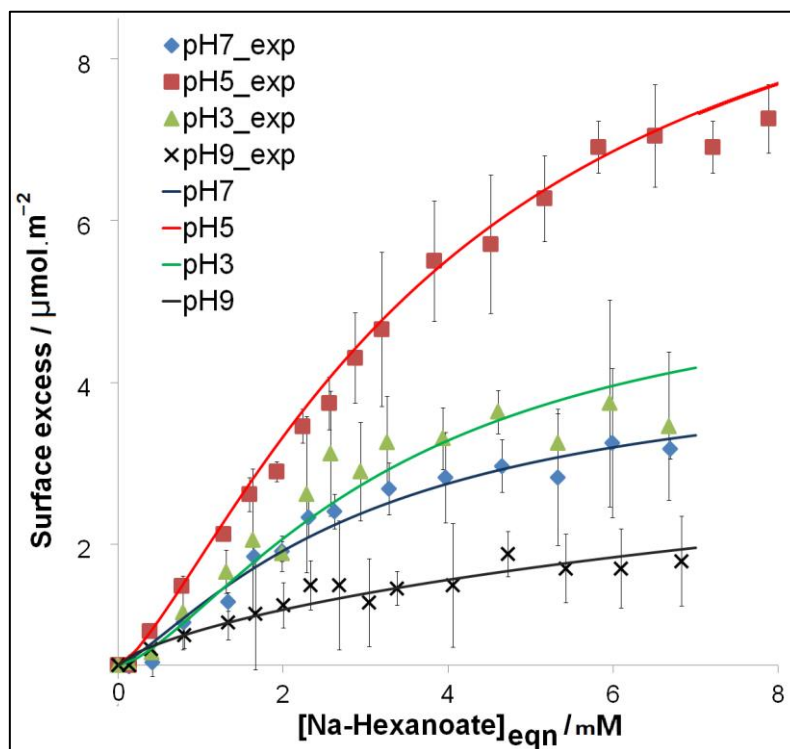
Figure 3. (a) Adsorption isotherm of sodium hexanoate at pH 3, 5, 7 and 9 (40 ml, and 0.11 g \alpha – alumina powder) measured by solution depletion method with non-Langmuir (S-shape) theory. (2-column fitting, colours for both web and paper)
