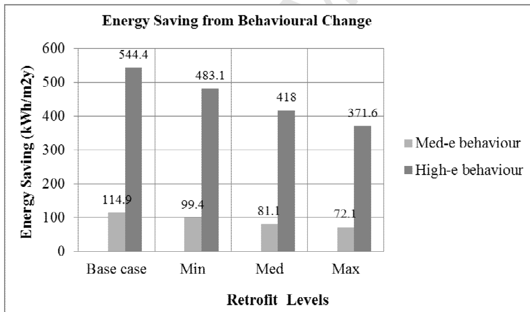
Fig.8. Energy saving comparison among different retrofit levels from behavioural change (Low-e behaviour is the baseline for med and high behaviour to change).
