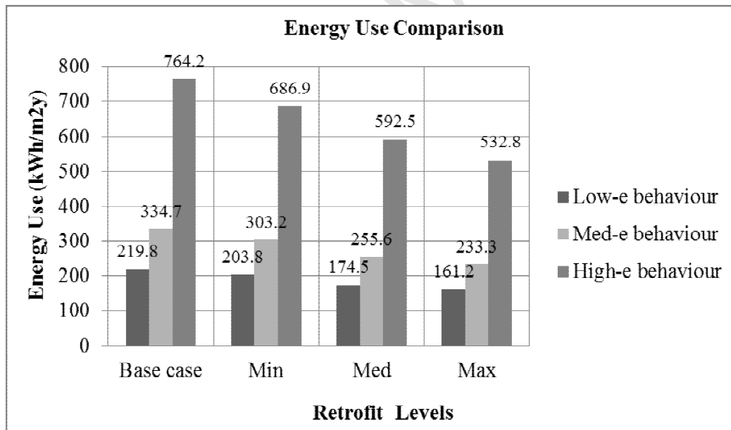
Fig.6. Energy use comparison among different retrofit levels with three behavioural scenarios
