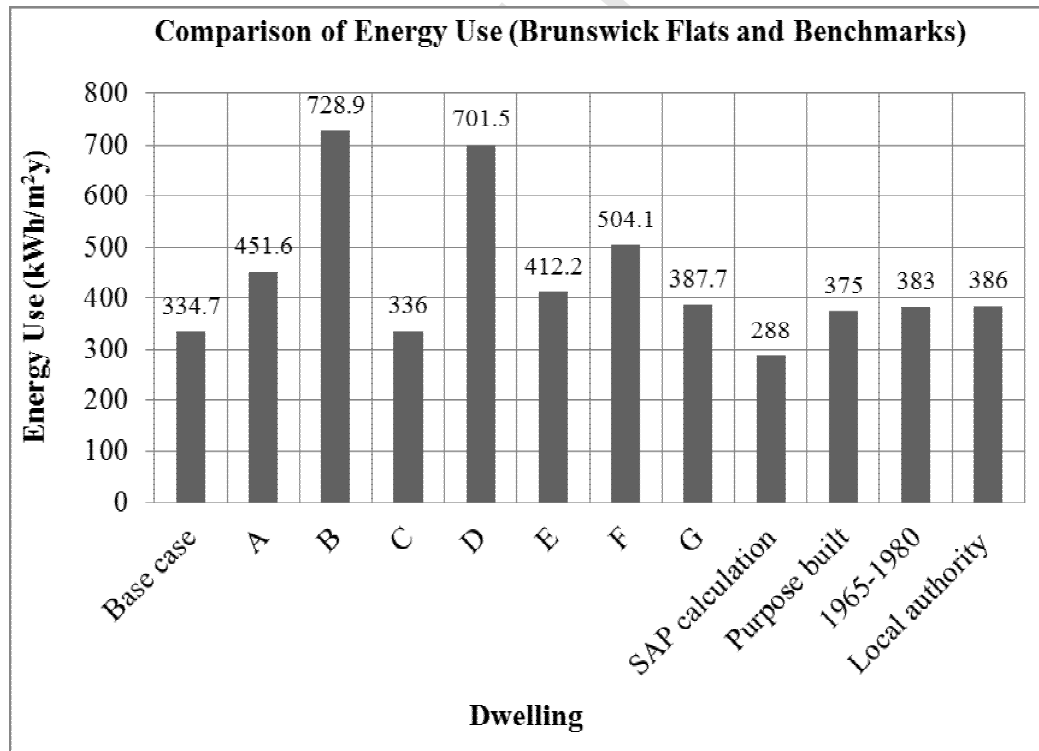
Fig.4. Comparison of energy use in the Brunswick flats to other benchmarks.
