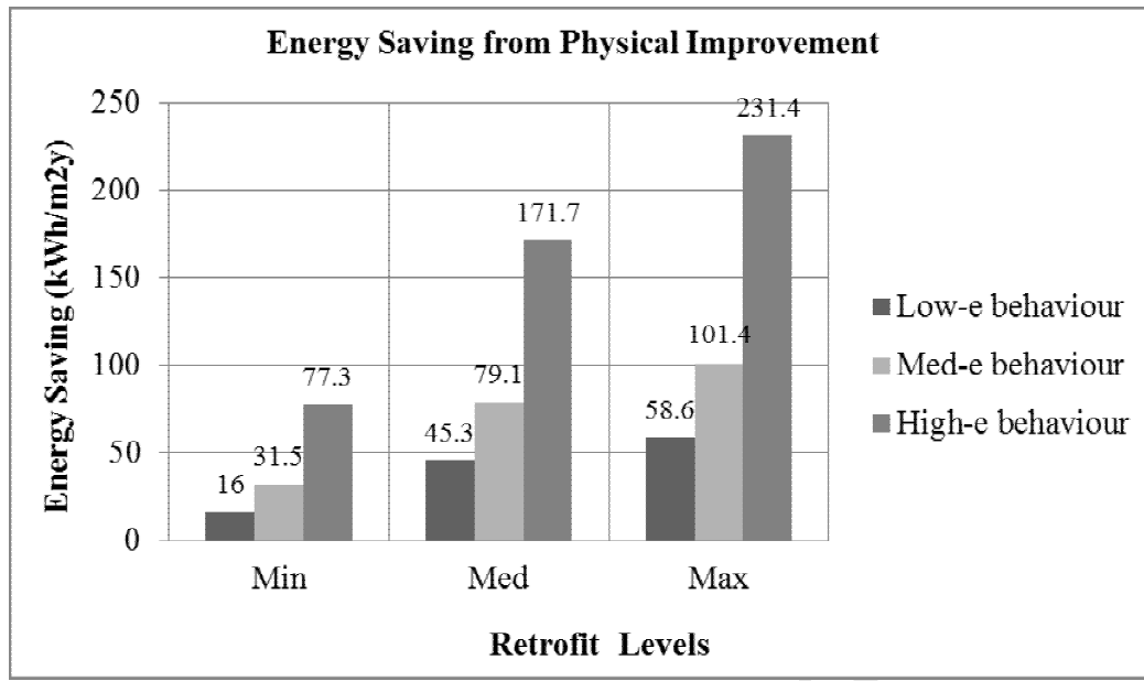
Fig.7. Energy saving comparison from physical improvement at three behavioural scenarios
