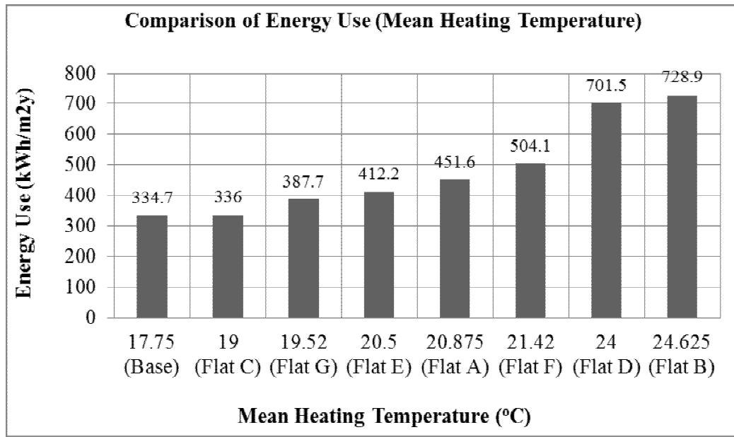
Fig.5. Comparison of energy use for mean heating temperature in the Brunswick flats.
