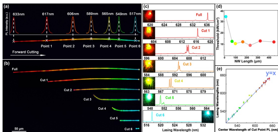
Figure 3. Defining lasing wavelengths widely on an individual bandgap-graded NW. (a) Real-color image of a bandgap-graded NW with 6 cut points determined by localized PL spectra. The NW has a diameter of \sim 450 nm and a length of 435 \mu\text{m} . (b) Real-color images of the NW after being cut at point 1 to point 6 sequentially. (c) Lasing spectra obtained from NW Full to Cut 6 are shown in (b). The colorful spots shown in each spectrum correspond to the real color image of the end emission of each NW at pump density above threshold. (d) Lasing threshold versus NW length of NW Full to Cut 6. (e) Lasing wavelengths versus PL center wavelengths measured from five bandgap-graded NWs and each NW is cut step-by-step for variable wavelength lasing emission. Colorful rectangular: experimental data; blue line: function y=x as a guide.
