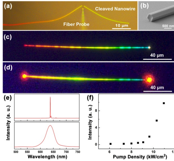
Figure 2. Micromanipulation and optical measurements of bandgap-graded NWs. (a) An optical microscope image of a NW being cut by a fiber probe. (b) Scanning electron microscope image of one endfacet of the cleaved NW shown in (a). (c, d) Real-color optical microscope images of a NW with a diameter of \sim 500 nm and length of \sim 170 \mu\text{m} under low and high pump density, respectively. (e) The spontaneous emission spectrum (bottom) and lasing spectrum (top) collected from the left end of the same NW as in (c) and (d), respectively. (f) Integrated output power as a function of pump density.
