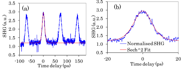
Fig. 3. Colinear autocorrelations of the pulse train emitted by the hybrid mode-locked MLLD, showing (a) a train of peaks of equal heights, and (b) a sech-squared fit to the zero delay peak corresponding to a pulse duration of 7.8 ps.
