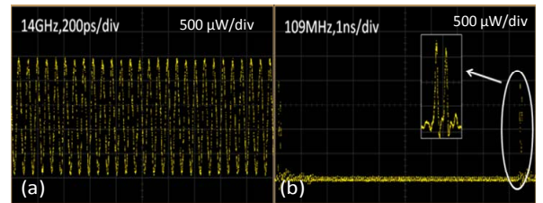
Fig. 5. Sampling oscilloscope traces of (a) an unmodulated pulse train at a repetition rate of 14 GHz (200 ps/div), (b) a modulated pulse train at 109 MHz (1 ns/div).
