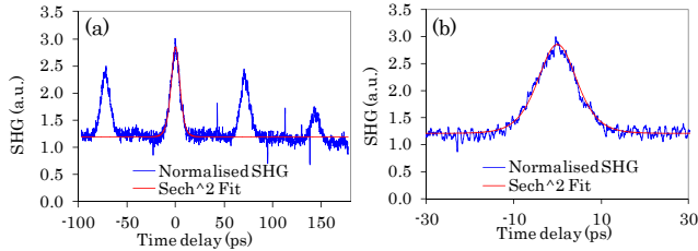
Fig. 6. Collinear autocorrelations of a modulated and amplified pulse train. (a) group of peaks and (b) zero delay peak.
