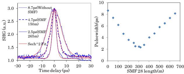
Fig. 4. Colinear autocorrelation traces after dispersion compensation in different lengths of SMF-28 fiber. The shortest measured pulse width is 2.4 ps at a fibre length of 325 m.
