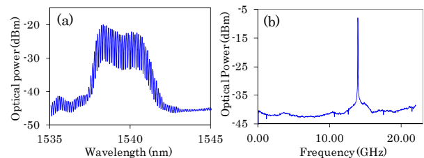
Fig. 2. (a) Optical spectrum with a centre wavelength of 1540 nm and a spectral width of 2.54 nm (b) RF spectrum of the laser output, with a peak frequency of 13.94 GHz.
