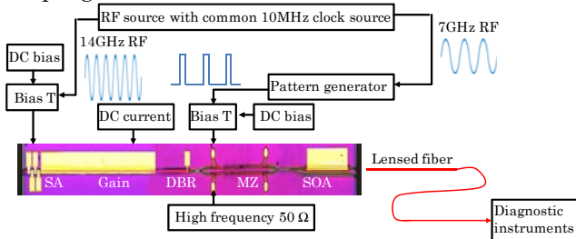
Fig. 1. A microscope image of the integrated device and a schematic diagram of the drive electronics used for hybrid modelocking, modulation and amplification of the pulse train.
