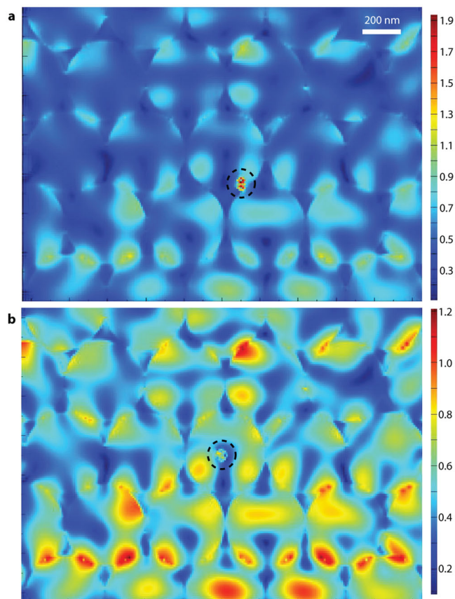
Figure 7. The simulated electric field distribution for gold nanoparticle (in the black dashed circles) modified BiVO 4 inverse opal at \lambda = 533 nm. The 20 nm gold nanoparticle is either a) on the inverse opal wall, or b) in the centre of one of the pores in the inverse opal away from the wall.
