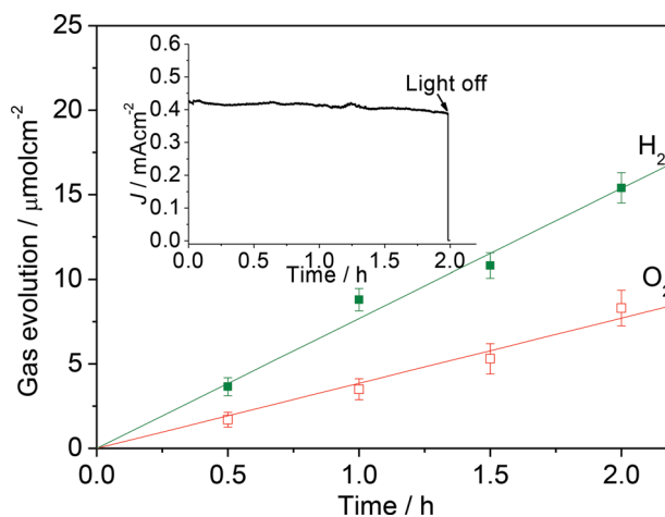
Figure 8. Gas evolution and the corresponding photocurrent transit (inset) of the io-Mo:BiVO 4 (260)/AuNP photoanode at an applied potential of 0.6 V (vs RHE).
