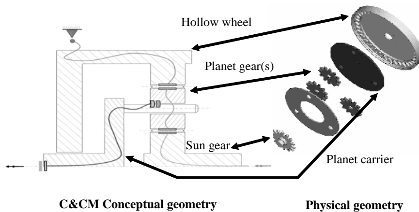
Figure 1. Planetary gear modelled using C&CM
