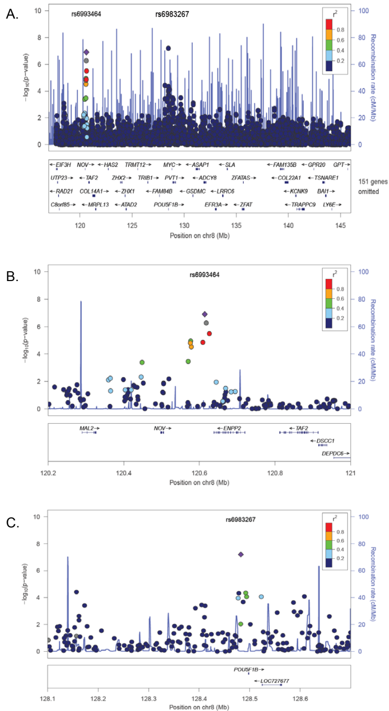
Figure 1 Individual GWAS top results and meta-analysis results for 8q24 region. (A) -\log_{10}(p\text{-values}) from meta-analysis using Fisher's method of the 8q24 region; (B) -\log_{10}(p\text{-values}) from meta-analysis for the region around NOV and ENPP2 . Purple diamond = rs6993464; gray = no LD data available in HapMap Phase II. Other colors indicate level of LD with rs6993464. (C) -\log_{10}(p\text{-values}) from meta-analysis using Fisher's method for the region around rs6983267. Purple diamond = rs6983267; colors indicate level of LD with rs6983267.
