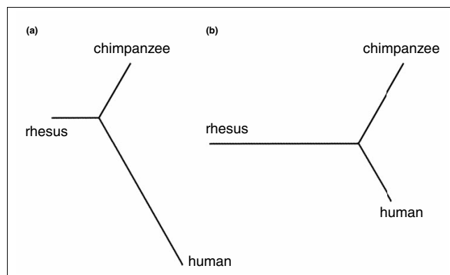
Figure 3 Divergence in metabolite abundance on the human and chimpanzee lineages. The trees are based on the abundance measurements of (a) 9 metabolites with significant concentration difference between human controls and schizophrenia patients and (b) 12 metabolites with no difference between these two groups. The trees were built using a neighbor-joining algorithm.
