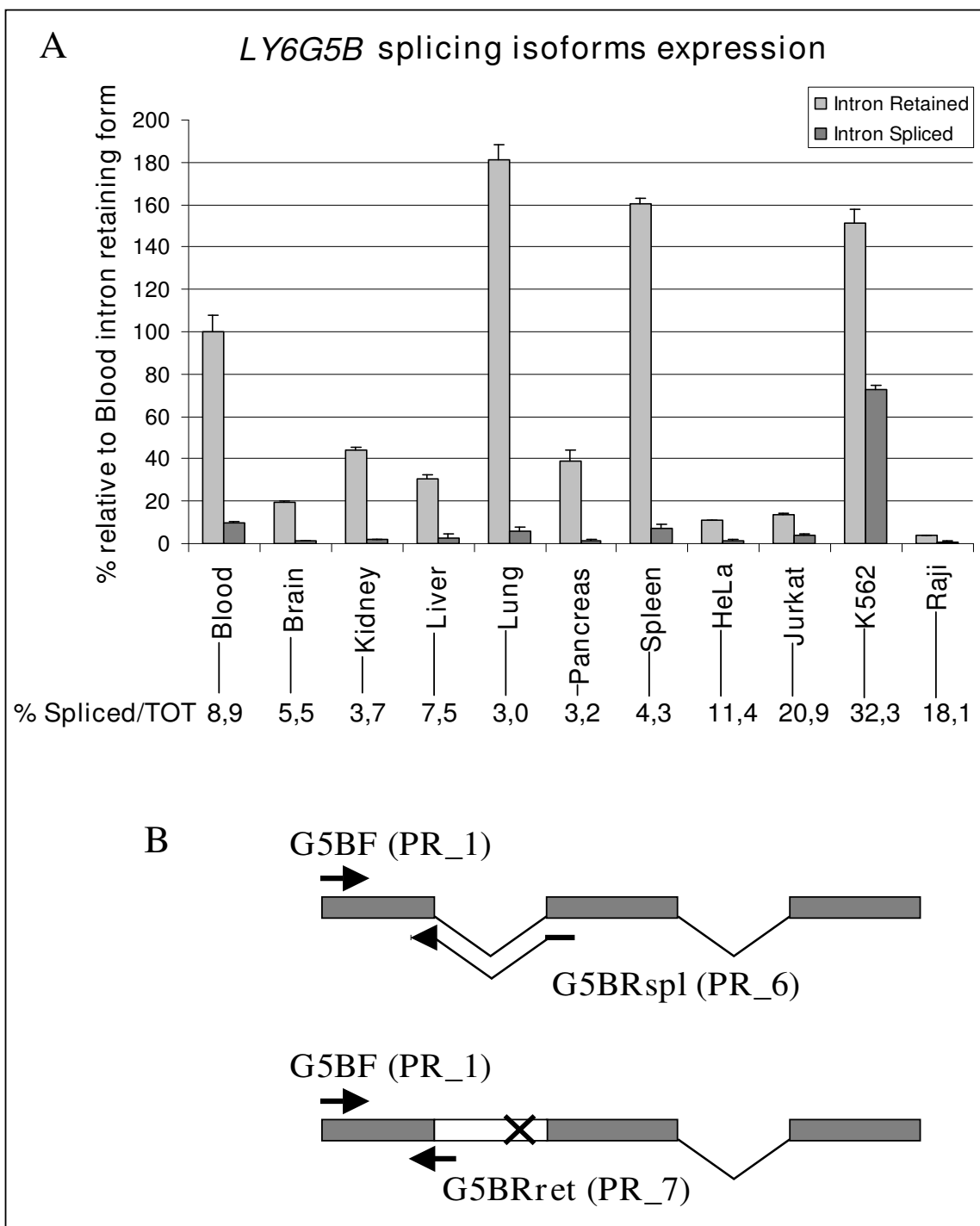
Figure 1 Differential real time RT-PCR assay for the two LY6G5B splice isoforms in a panel of human tissues and cell lines. (A). Data are expressed in relation to the percentage of the intron-retained form expressed in blood. Numbers below the graph represent the percent of the correctly spliced isoform of LY6G5B relative to the total expression of the gene in each sample. PCR reactions were run in triplicates. (B) Schematic representation of the primer design for the differential assay. Forward primer (PR_3) is shared while reverse primers (PR_6 and 7) share only 4 nucleotides at the end of the first exon. X indicates the premature stop codon.
