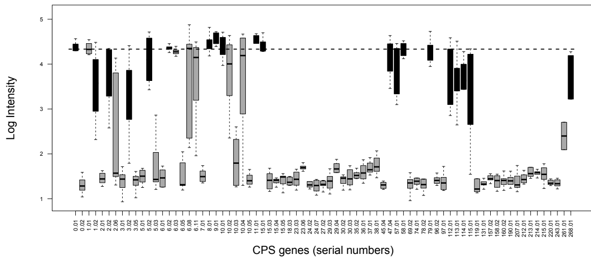
Figure 1 Boxplot of CPS probe log intensities for an array testing a sample containing one serotype. Plot of the log probe intensities for the cps genes from an example of a Streptococcus pneumoniae serotyping microarray experiment testing a sample containing only one serotype. The serial numbers of the genes are given on the horizontal axis. Only the top 75 genes (out of a total of 432 genes), with the highest mean probe log intensity are plotted for clarity. The cps genes found in the particular serotype being tested by this microarray experiment are marked in black. Note that some of the cps genes not expected in this serotype have elevated intensities. This reflects cross-hybridization of probes. The horizontal dotted line marks the median log intensity of the 6824 S. pneumoniae SpTIGR4+R6 genome probes.
