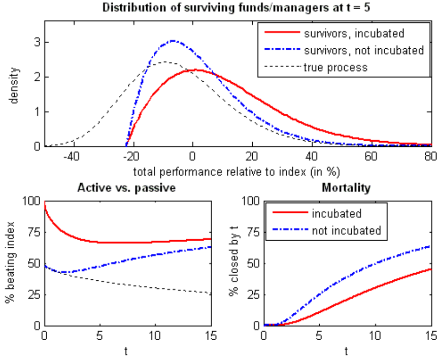
Figure 2: Survivors' vs. true performance process. The top graph's horizontal and vertical axes are 100 \cdot (\hat{a} - 1) and f(\hat{a}) , respectively, where f denotes the densities of a_6^* ( \kappa = 1 ), a_5^* ( \kappa \downarrow 0 ) and a_5 ; the legend also applies to the bottom left graph. Parameters: f = 0.01 , \sigma = 0.08 , c_0 = 1 , c = 0.775 and \mu_\kappa = 0 . If incubated, \sigma_\kappa = 0.15 . If not, \sigma_\kappa \downarrow 0 .
