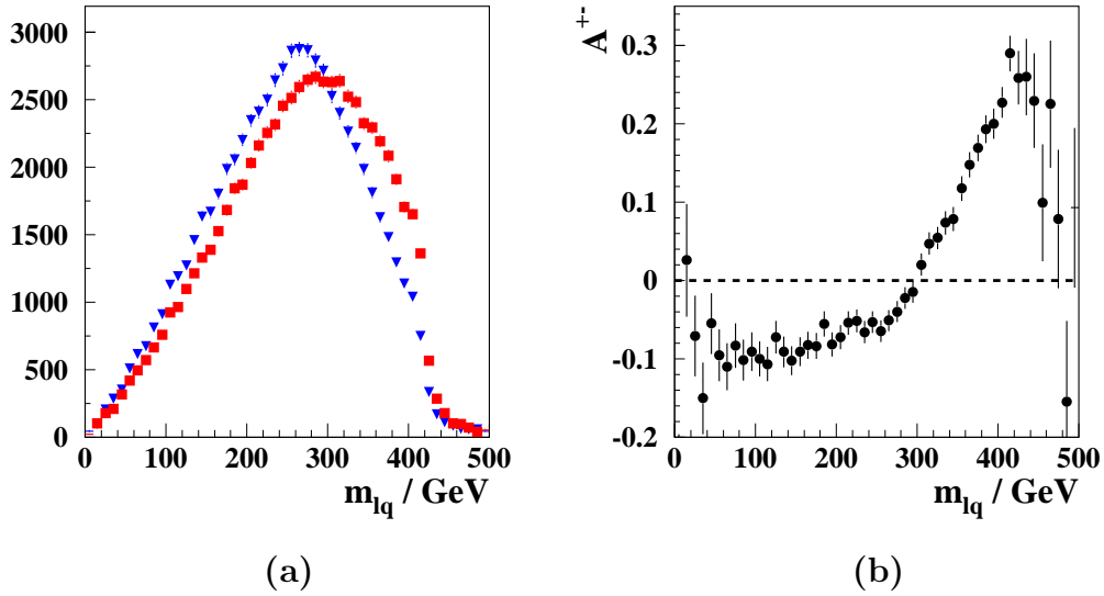
Fig. 6. (a) The l^{+} q (squares) and l^{-} q (triangles) invariant mass distributions, and (b) the charge asymmetry A^{+-} (eq. 11) at the parton level. These distributions have folded-in the indistinguishability of the near and far leptons, and quark vs. anti-quark jets.
