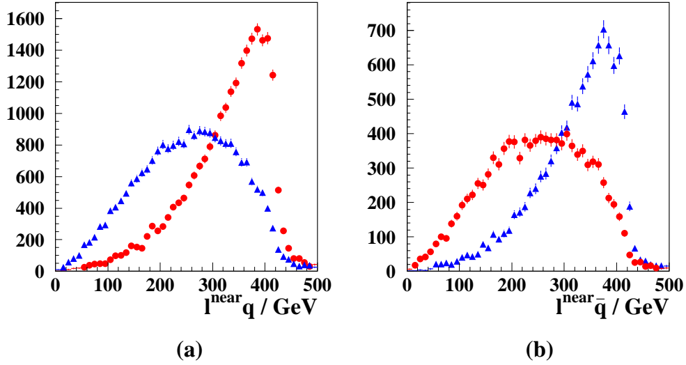
Fig. 3. Invariant mass distributions of (a) l^{\text{near}}q and (b) l^{\text{near}}\bar{q} , at the parton level. The triangles are for a negatively charged near lepton, while the circles are for a positively charged near lepton. For the test point the on-shell kinematic maximum is 413.4 GeV. Note that these distributions cannot be measured directly by the experiment.
