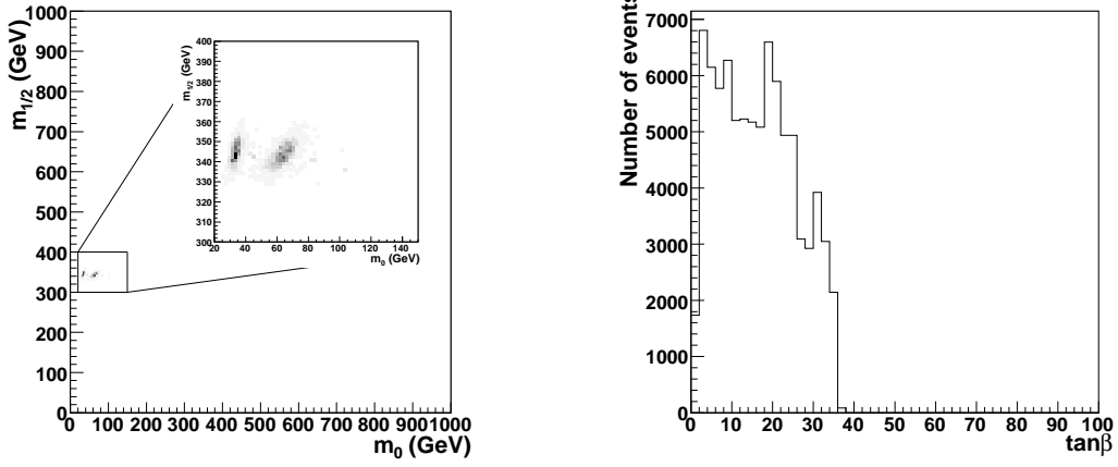
Figure 17: The region of mSUGRA parameter space consistent with the endpoint measurements of section 2, without the assumption that the neutralinos and slepton in the squark decay chain have been correctly identified. For full details, see text. Results are shown for positive \mu .
