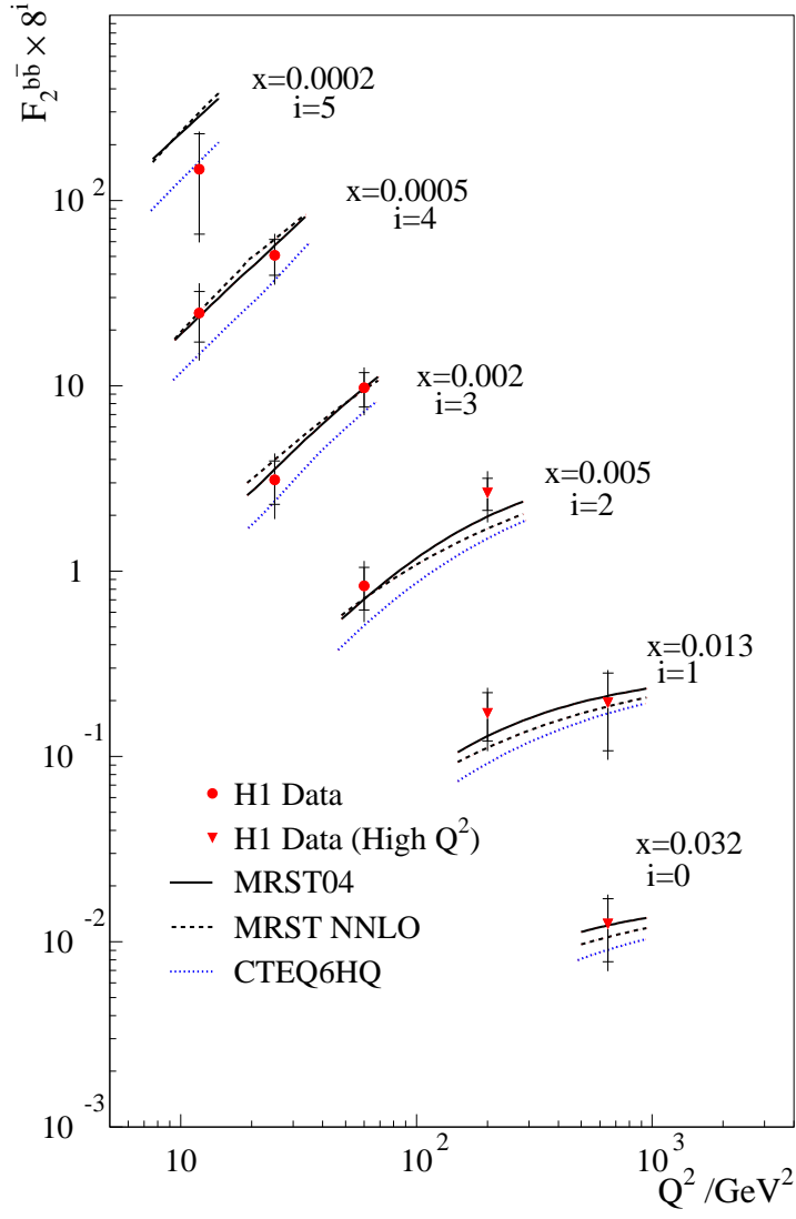
Figure 4: Comparison of the NLO and NNLO predictions for F_b^c(x, Q^2) compared with H1 data.
