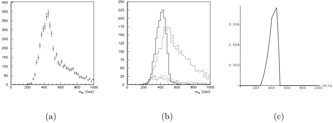
Fig. 3. Three sets of m_{qt} -threshold distributions for the CMSSM mSUGRA model described in the text. (a) shows what might be seen in a typical LHC experiment after the cuts described in the text. Figure (b) shows (a) broken down into the four components which contribute to it. These are (1) a narrow component coming from events in which the jet was correctly identified (solid line), (2) a broad component in which the jet was incorrectly identified (dashed line), (3) a small component representing the contribution from all SUSY sources which have nothing to do with the desired chain (dotted line), and finally (4) a small component from all SUSY sources which pass opposite-sign different-family versions of the cuts (dot-dashed line). The shape of component (4) matches the shape of (3) nicely and is added with negative weight in (a) to subtract component (3). Figure (c) shows the shape of the m_{qt} -threshold distribution as predicted in the text using the masses m_{\tilde{\chi}_1^0} = 121.5 , m_{\tilde{l}} = 157.2 , m_{\tilde{\chi}_2^0} = 233 and m_{\tilde{q}} = 656 GeV.
