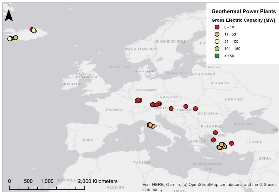
Figure 16 Geothermal Power Plants from [45]. Own illustration of Europe.
