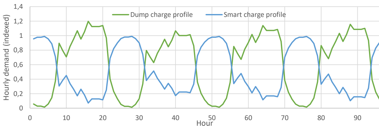
Figure 19 Electric vehicle profile example from United States 2001 [65]
