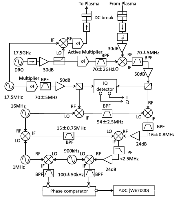
FIG. 2. Schematic of millimeter-wave interferometer system.
