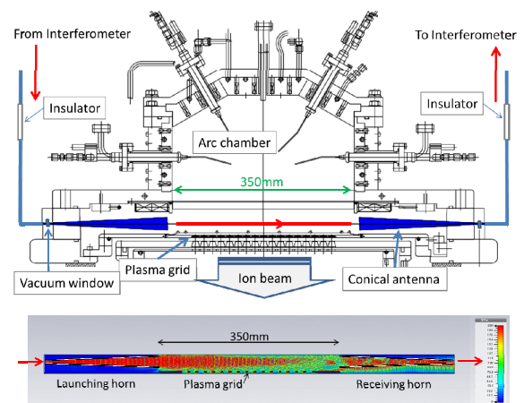
FIG. 1. (Color online). Schematic of cross section of arc chamber (350 x 220 mm). The traveling path of millimeter-wave is around 350 mm and the line of sight is around 18 mm far from the plasma grid surface. In order to protect the charging when the operation of high voltage is applied to the negative ion source, the Teflon rod as an insulator is inserted into the waveguide transmission line. The bottom figure shows the calculated propagating beam pattern.
