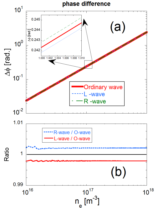
FIG. 5. (Color online). (a) Calculated phase difference as a function of electron density. In each calculation, it is assumed that the polarization is ordinary mode (red solid line), L-wave (blue dotted line), and R-wave (green dashed line). (b) The ratio of R-wave and ordinary wave (blue dotted line), and that of L-wave and ordinary wave (red solid line).
