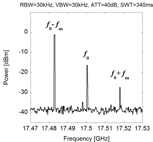
FIG. 3. Frequency spectrum of single-side-band modulating output.
