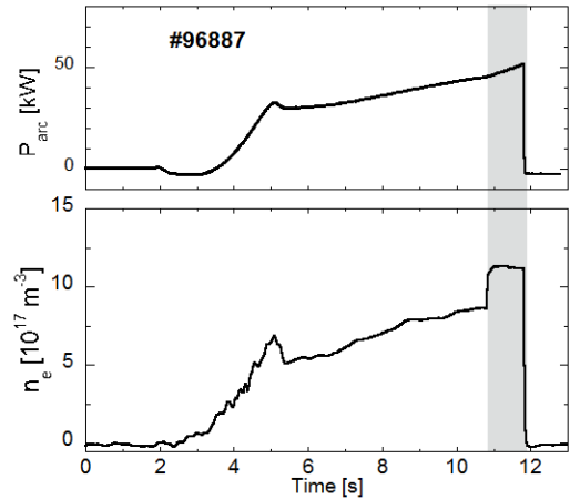
FIG. 6. Temporal behavior of the input power to arc chamber (top) and the line-averaged electron density (bottom). After t=10.8 s (hatching area), high voltage is applied to extract the negative ion beam.
