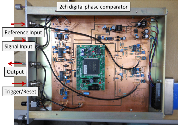
FIG. 4. (Color online). Photograph of digital phase comparator.
