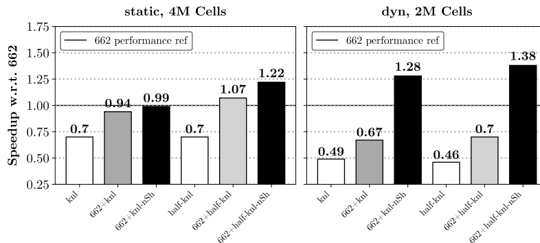
Fig. 6. Speedup in combining a 662 node and a KNL by using nSharma
