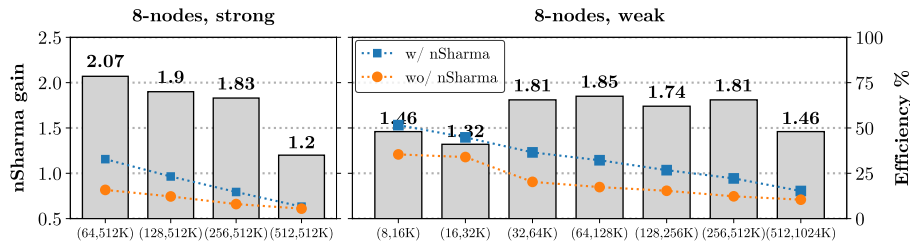
Fig. 5. nSharma gain Efficiency (w/ and wo/ nSharma) with dynamic loads for 8 Stampede2 KNL nodes
