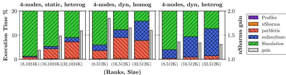
Fig. 3. Execution time percentage breakdown for 4 nodes
