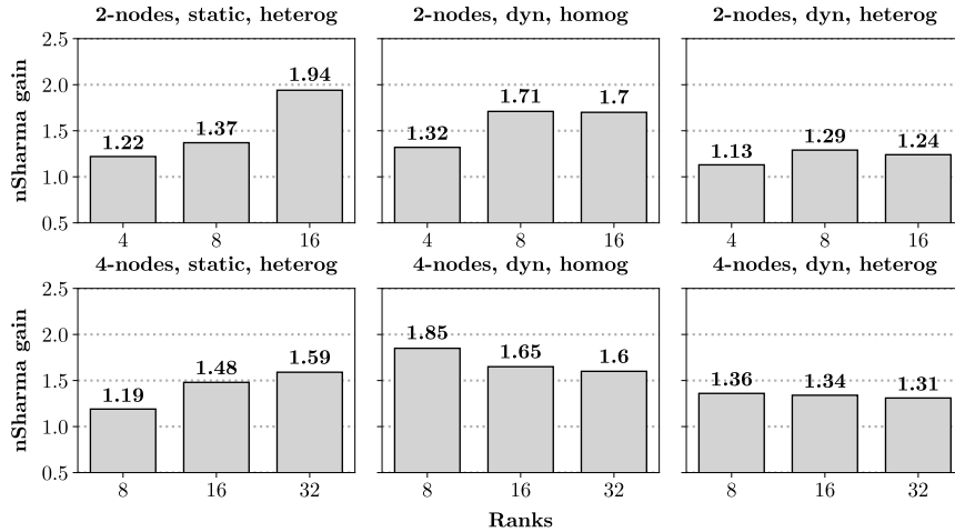
Fig. 1. nSharma gain with Homogeneous and Heterogeneous I configurations on SeARCH, with size 512K for dynamic and 1024K for static
