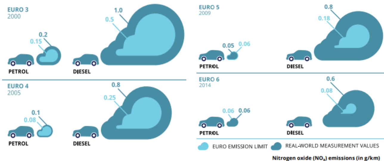
Fig. 2: EU limits and real-world nitrogen oxide (NO x ) emissions (in g/km): comparison between gasoline and Diesel cars, according to the European Environmental Agency [15].
