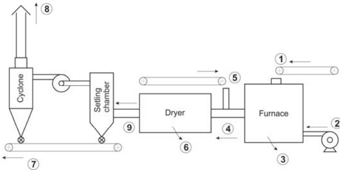
Fig. 6: Schematic view of the biomass dryer
