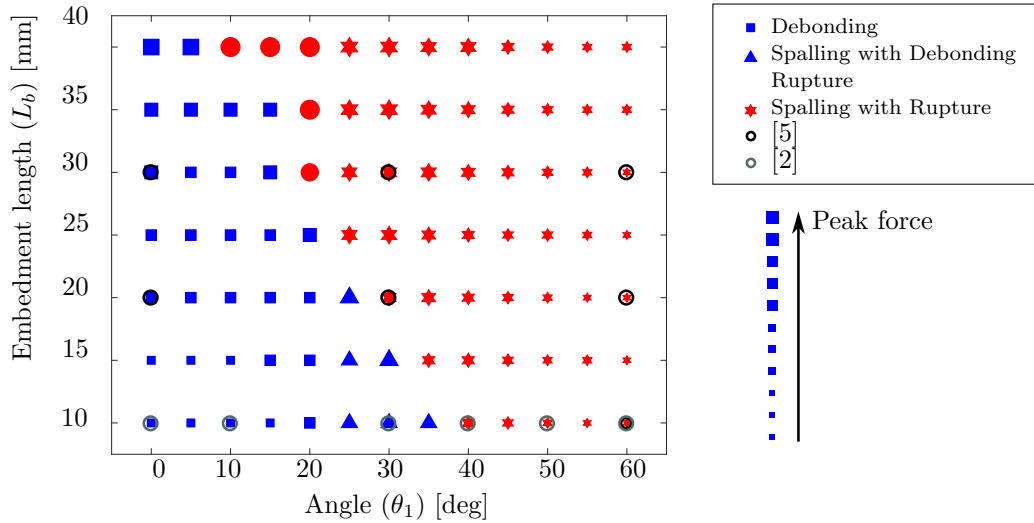
Figure 7: Failure mode map in the \theta_1 and L_b space for the SFC from [17]. The black and grey circles shows the data from [5] and [2] where similar configurations were tested.
