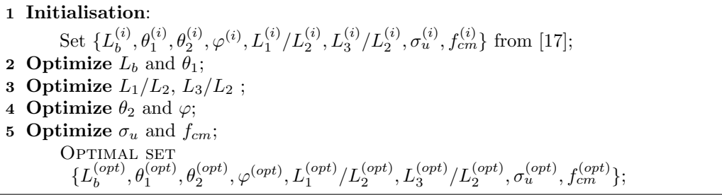
Figure 5: Optimization strategy used to get the optimal values of the geometric and material parameters of the FRC composite.
