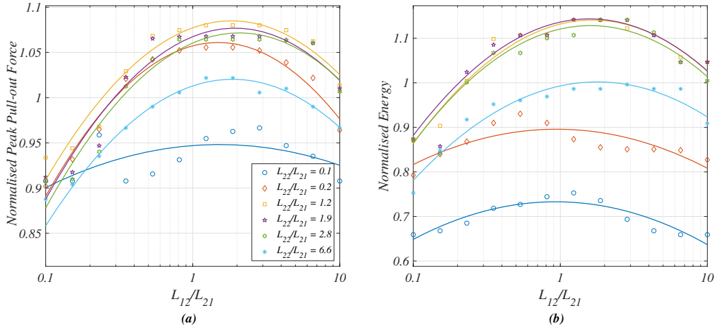
Figure 9: Peak pull-out force (a) and energy absorption capacity (b) in terms of L_1/L_2 \in [0.1, 10] and L_3/L_2 \in [0.1, 6.66] . The peak force and the energy are normalised with respect to the optimal configuration in Figure 6, which was achieved for L_1/L_2 = 9.8 and L_3/L_2 = 0.88 .
