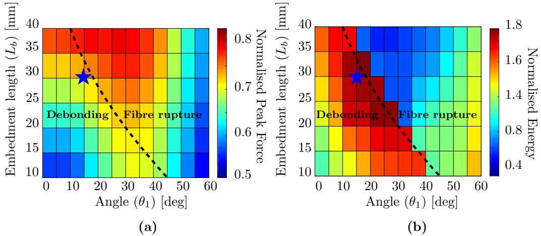
Figure 6: Contour plot of the peak pull-out force (a) and energy absorption capacity (b) for \theta_1 \in [0, 60] and L_b \in [10, 40] mm. The thick dashed lines show the transition between two failure modes given by Eq. (8): complete debonding of the fibre from the matrix or fibre rupture. The blue star indicates the optimal configuration chosen to carry out the sensitivity analysis in Sec. 3.2.
