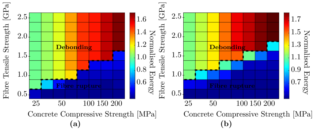
Figure 12: Contour plot of the normalised energy for fibres oriented at 15^\circ (a) and 60^\circ (b) fibres for a concrete strength in the range [25, 200] MPa and fibre tensile strength in [0.5, 2.5] GPa. The thick dashed lines show the transition between two failure modes: complete debonding of the fibre from the matrix or fibre tensile rupture.
