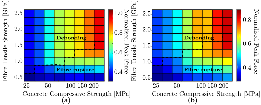
Figure 11: Contour plot of the normalised peak force for fibre oriented at 15^\circ (a) and 60^\circ (b), for a concrete strength in the range [25, 200] MPa and fibre tensile strength in [0.5, 2.5] GPa. The normalisation is carried out for a fibre with P_{fu} = \sigma_u A equal to 530 N.
