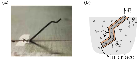
Figure 1: (a) Picture of the real specimen used in [17]. (b) Schematic representation of the specimen with the different fibre segments used for modelling.
