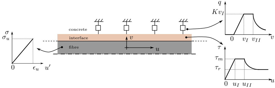
Figure 2: Constitutive laws for the three components of the fibre reinforced concrete, where just half of the system is shown due to the symmetry with respect to the dot-dashed line.
