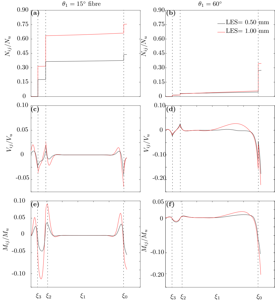
Figure 8: Normalised axial and shear forces and bending moment along the fibre length for a fibre with \theta_1 = 15^\circ (a,c,e) and \theta_1 = 60^\circ (b,d,f), where LES is the load end slip. \xi_i represents the curvilinear abscissa along each fibre segment.
